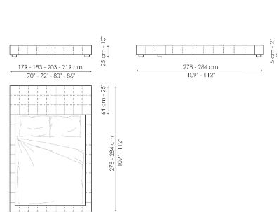
Squaring isola Width: 179-183-203-219cm Depth: 278-284cm Height: 25cm
