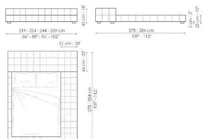
Squaring penisola variante B Width: 219-224-244-259cm Depth: 278-284cm Height: 45cm
