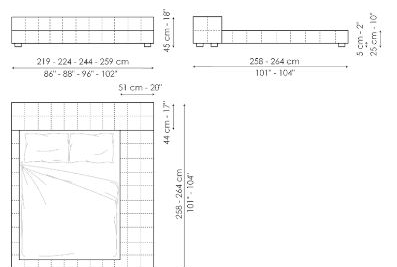
Squaring penisola variante A Width: 219-224-244-259cm Depth: 258-264cm Height: 45cm
