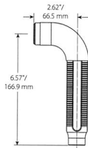
Long 90° elbow reducer
