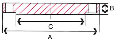
Blind Flange
