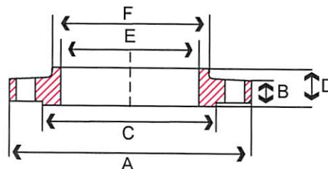
Slip-On Flange
