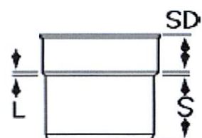
IPS HUB X SEWER SPIGOT ADAPTER
