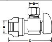
Angle Stop (Chrome Plated) Dimensions
