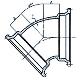
MJ x MJ Bend 45°
