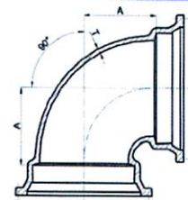
MJ x MJ Bend 90°
