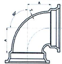
MJ x MJ Bend 90°
