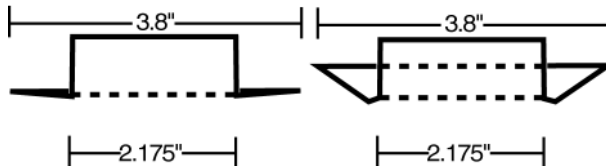
Flush Skirt adjustable 1/4" to 3/4" with short cup 1/4" to 1-5/8" with standard cup
