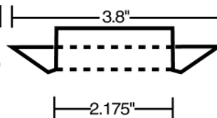
Short Taper Skirt adjustable 3/4" to 1" with short cup 3/4" to 1-7/8" with standard cup
