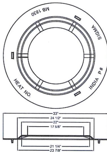
18" x 30" Adapter Ring Shipping Weight: 65 lbs.
