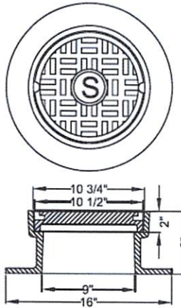
6" Lamphole Frame and Cover Shipping Weight: 50 lbs.
