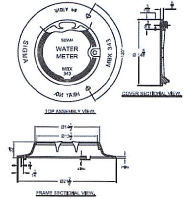
20" Meter Tile & Cover Shipping Weight: 39 lbs.
