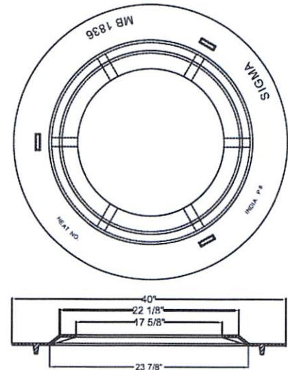
18" x 36" Adapter Ring Shipping Weight: 100 lbs.
