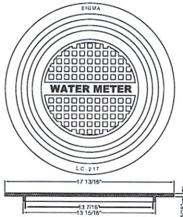
18" Chattanooga Meter Tile Plate Shipping Weight: 16 lbs.
