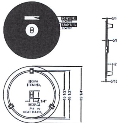
Meter Tile Cover Shipping Weight: 59.5 lbs.
