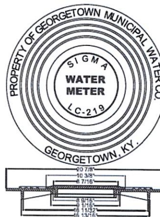
CI Outer and Inner Lid with Reader Lid "Georgetown Metro Water" Shipping Weight: 39 lbs.
