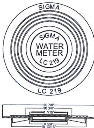
CI Outer and Inner Lid marked "Water Meter" Shipping Weight: 39 lbs.
