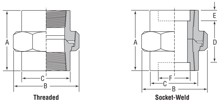
FIGURE 2125: Threaded Union
