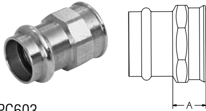
PC603 Adapter P x F – Brass Rod (*Wrot)
