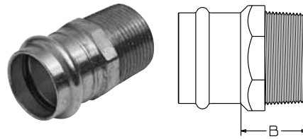
PC604 Adapter P x M – Brass Rod (*Wrot)
