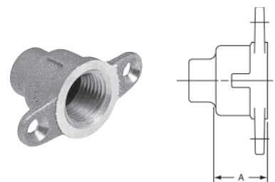
703-5 Special Drop Adapter C x F – Cast
