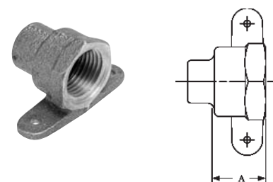
703-5B Drop Adapter C x F – Cast
