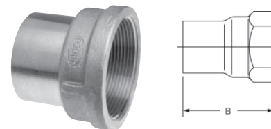
703-2 Fitting Adapter Ftg x F – Cast
