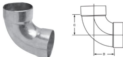
907 DWV 90° Elbow C x C – Wrot
