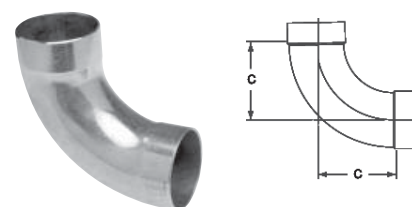
907-LT DWV 90° Long Radius Elbow C x C – Wrot
