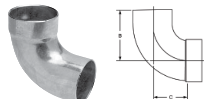
807-2 DWV 90° Fitting Elbow Ftg x C – Cast
