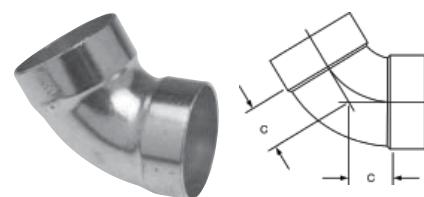
960 DWV 60° Elbow C x C – Wrot
