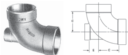
861-LH DWV 90° Elbow w/Low Heel Inlet C x C x C – Cast
