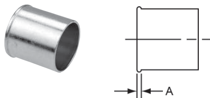
616 Fitted Plug Ftg - Wrot
