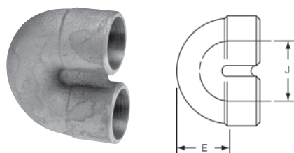
739 Return Bend - Closed C x C - Cast
