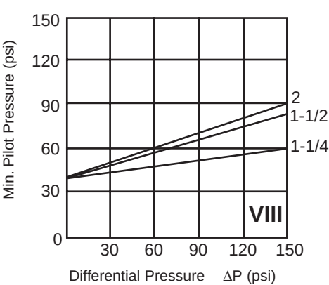
Normally Closed Valve - Entry Above Disc
