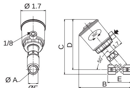
Normally Closed
