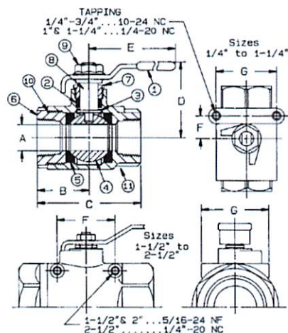
BRONZE FULL PORT BALL VALVE
