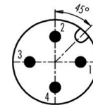
Female insert M12
