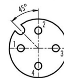
Female insert M12
