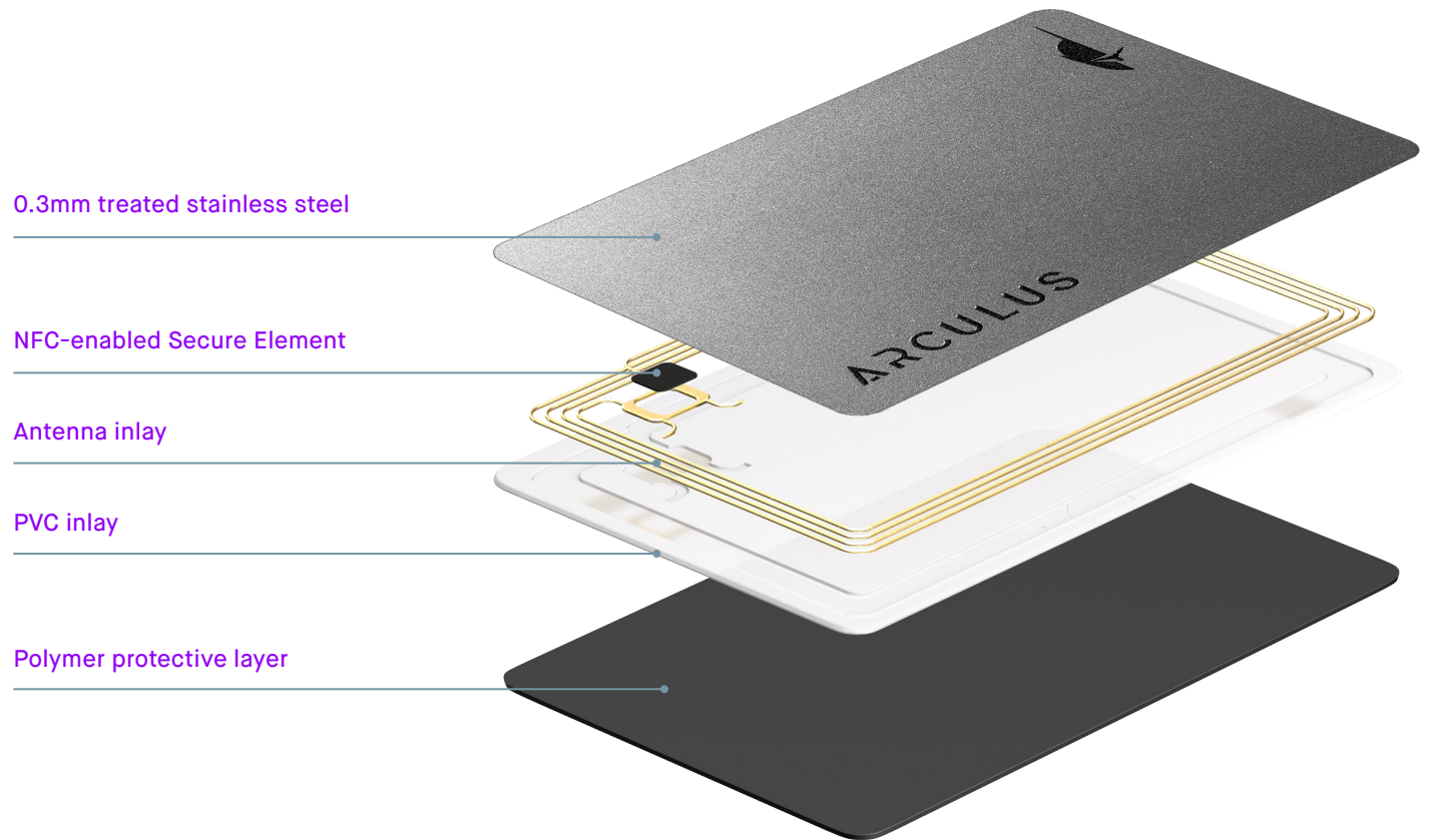
Figure 1: Components of the Arculus Card
