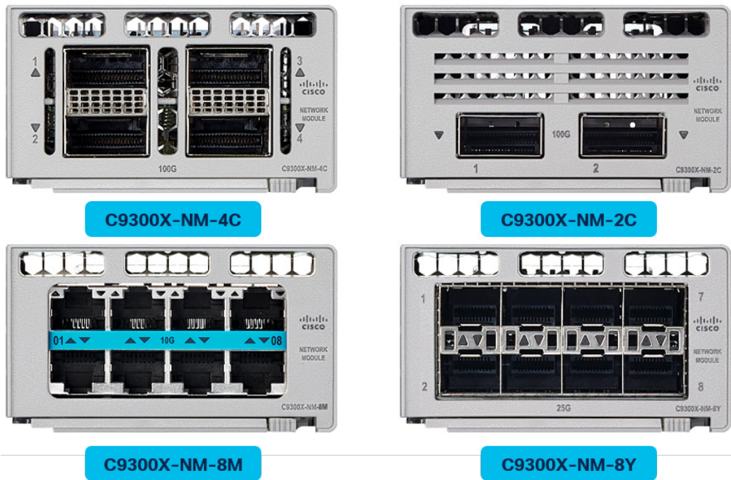
Figure 2. Cisco Catalyst 9300X network modules
