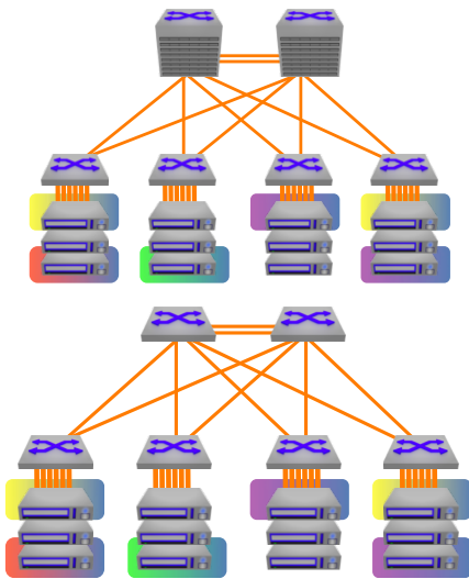
Arista Leaf-Spine Two-tier Network Architecture with 7060X and 7260X Series
