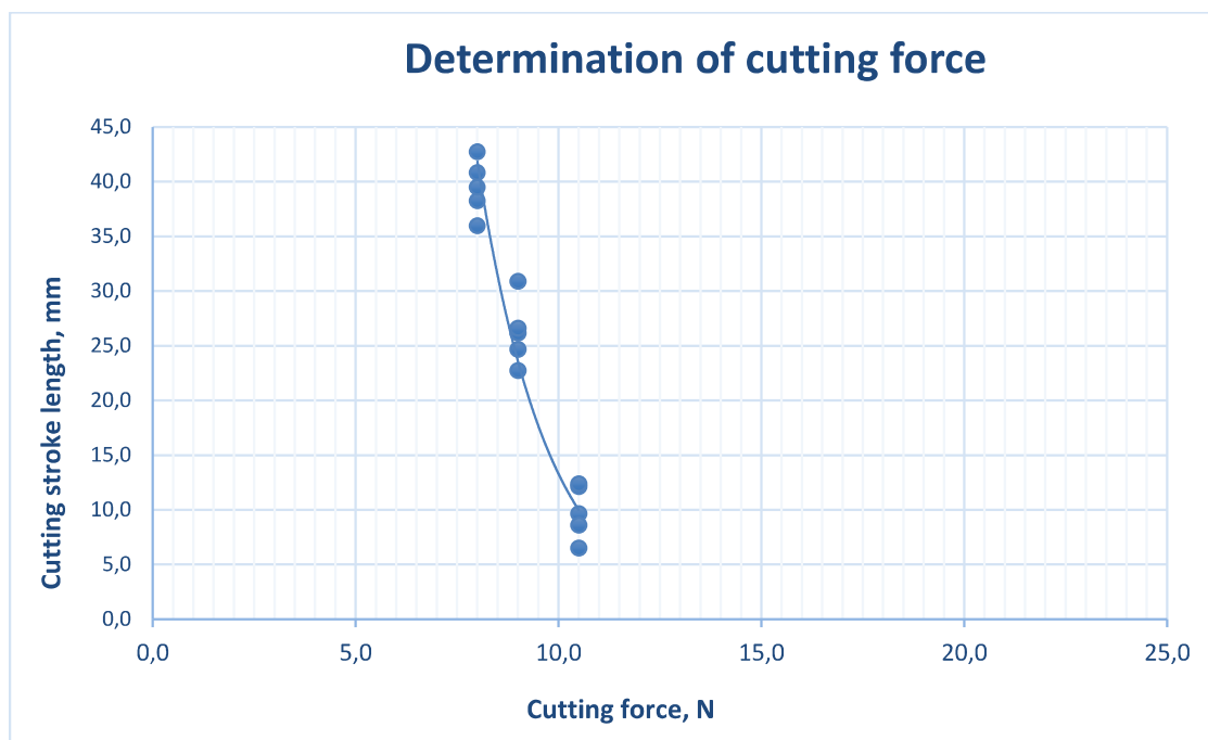
Picture 1: Recording of the cutting force in relation to the cutting stroke length with correction factor C and the resulting regression line
