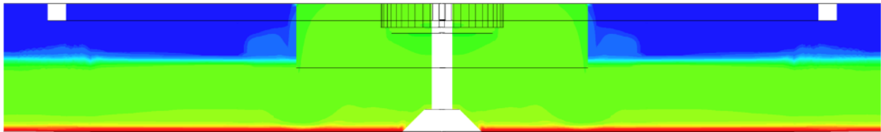
Figure 11: CFD model results for solids concentration of a clarifier. Colors are as follows: dark blue is 10 mg/L, light blue is 1,000 mg/L, green is 3,000 mg/L, and red is 6,000 mg/L.
