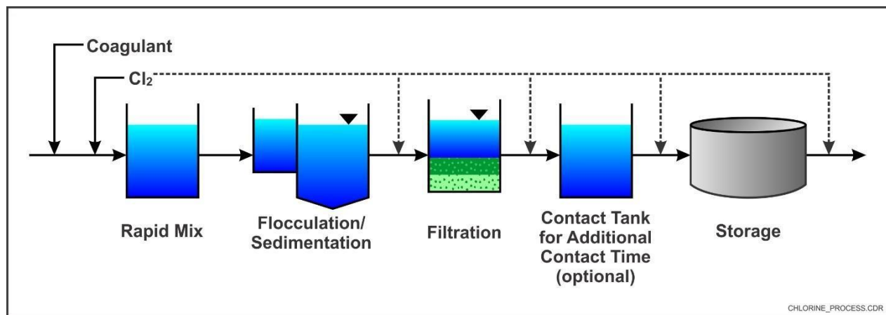
Figure 1: Water treatment system with sand filtration and chlorine disinfection.
