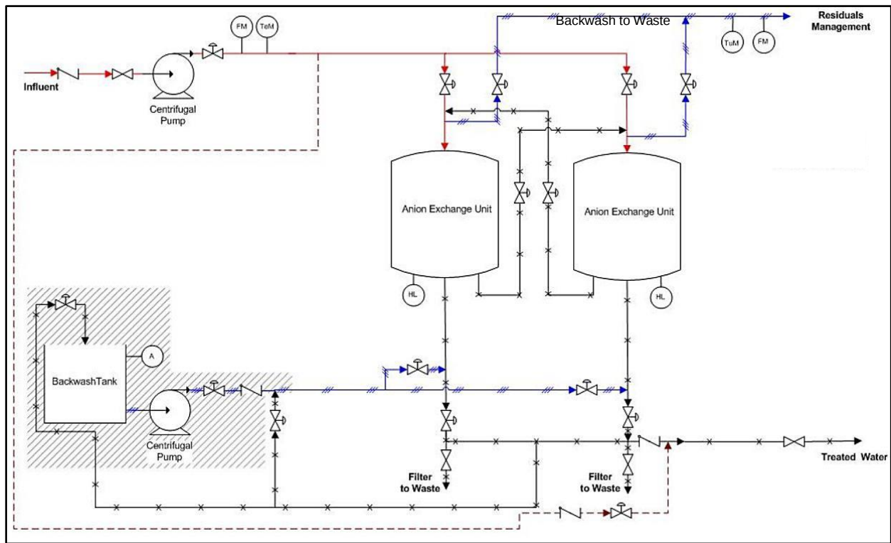
Figure 7: Example PFD with basic features. This drawing could be a starting point for creating a P&ID with control and communication details.
