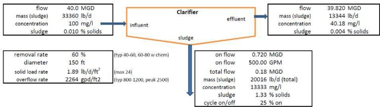
Figure 10: Example mass balance for a clarifier at peak flow. Note the mass of sludge entering the clarifier (33,360 lb/d influent) equals the mass leaving the clarifier (13,344 lb/d effluent plus 20,016 lb/d sludge).
