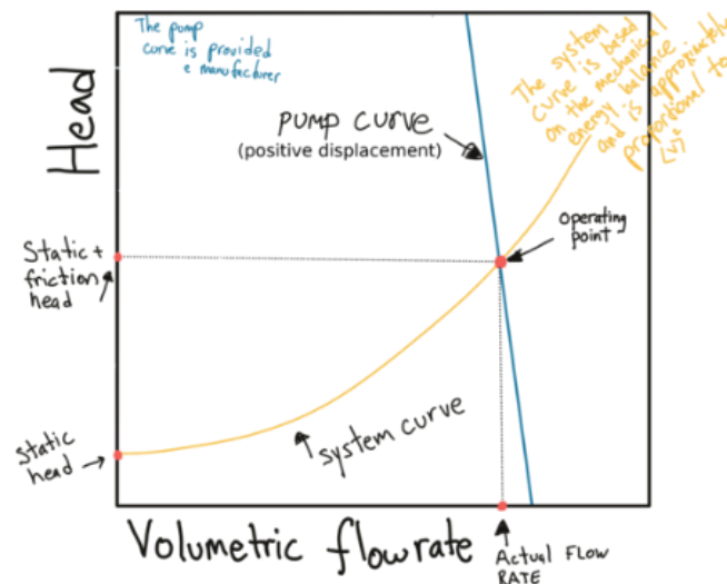
Figure 12: Pump and system curves with operating point based on field testing.
