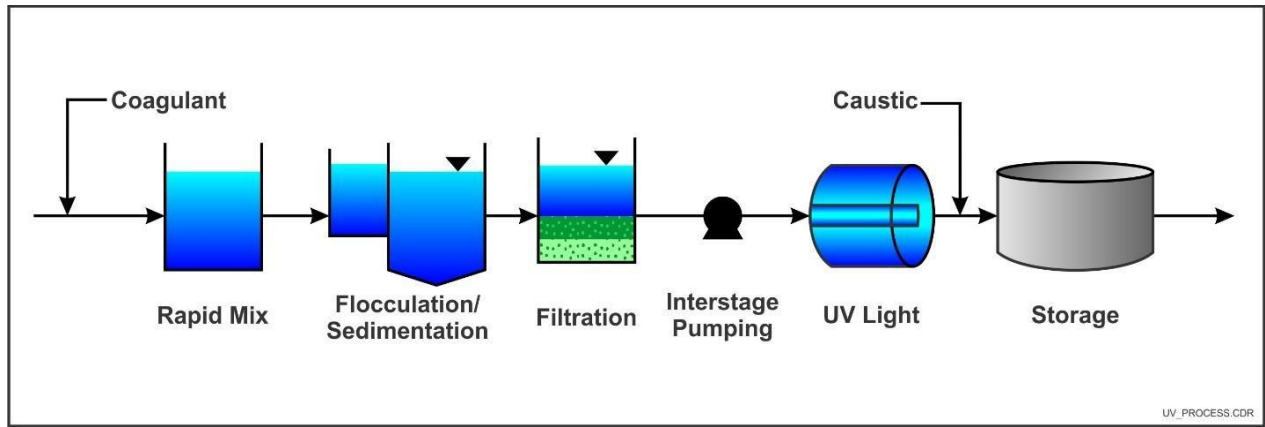
Figure 2: Water treatment system with sand filtration and UV disinfection.
