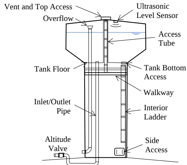
Figure 12: Typical tank features for a fluted column elevated storage tank.
