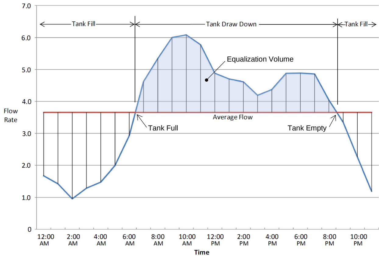
Figure 7: Example equalization curve with diurnal demand in blue and the average daily flow in red.
