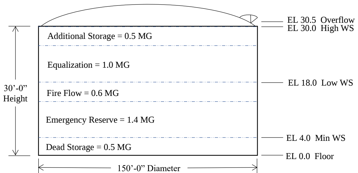
Figure 8: Profile of a 4 MG Tank with elevations and demand volumes.
