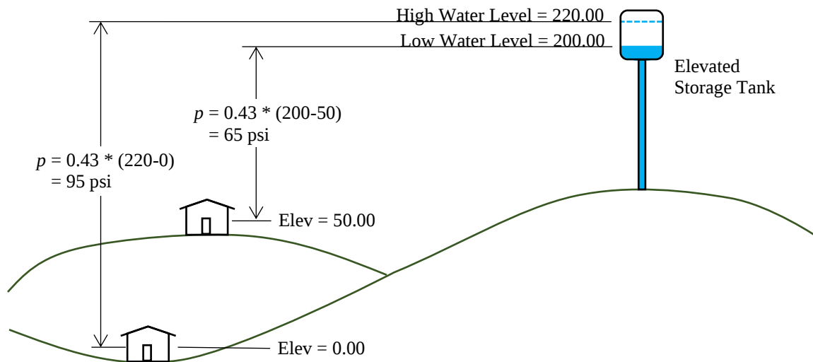
Figure 5: Water pressure ( p ) calculated for the buildings at the lowest and highest elevations in a community with an elevated storage tank.
