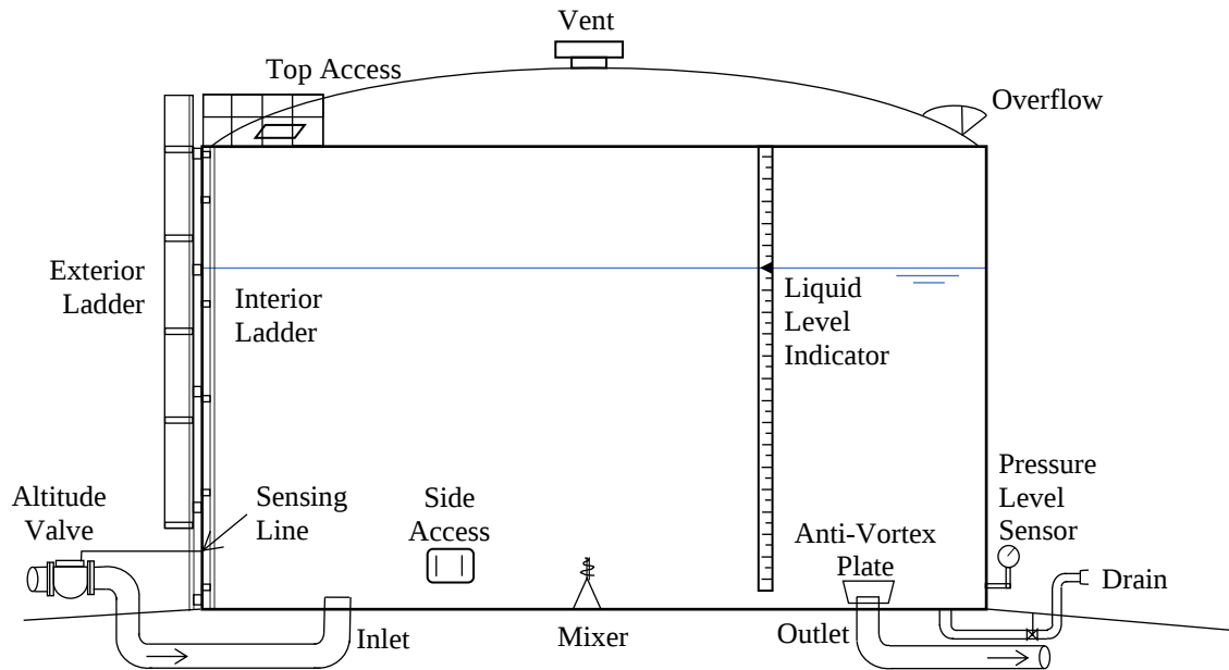
Figure 11: Typical tank features for a ground storage tank.
