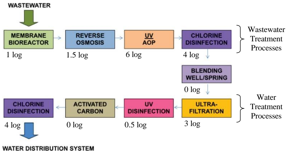
Figure 17: Block flow diagram for Example Problem 4. The virus log removal is stated for each process. Note that AOP stands for Advanced Oxidation Process.
