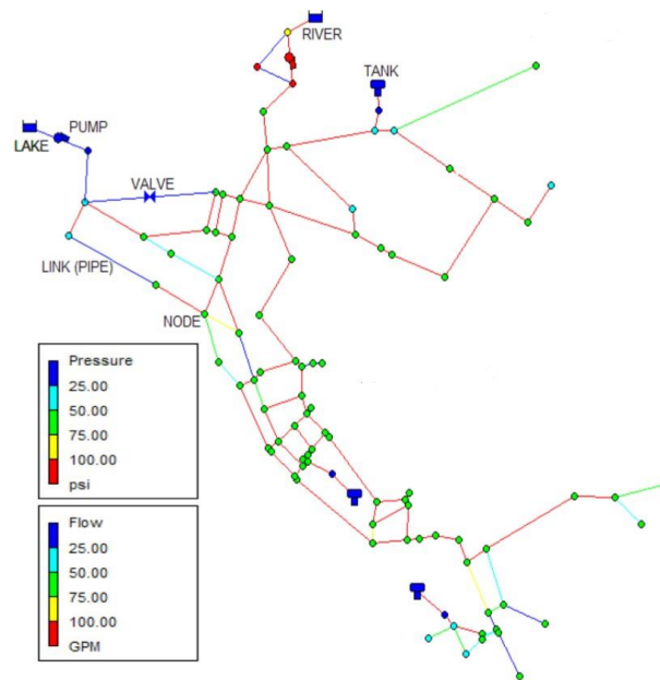
Figure 6: Example of a hydraulic model with the lines (pipes) colored for flow and nodes (branch connections) colored for pressure.
