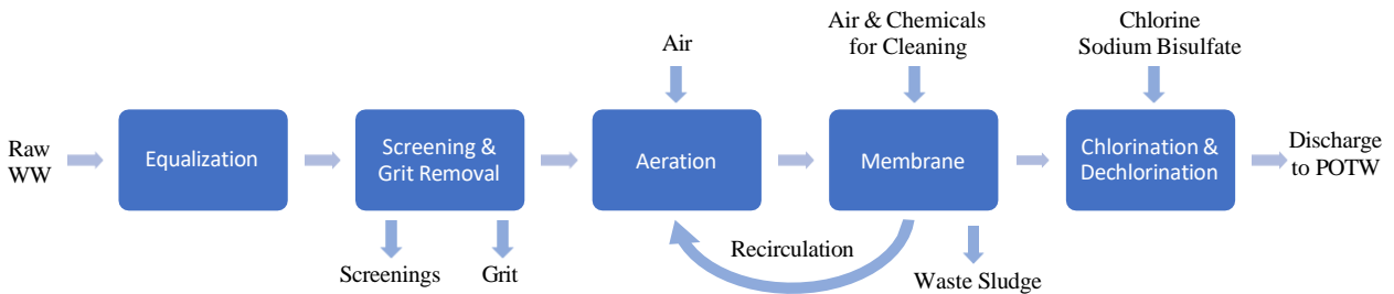
Figure 1: Wastewater treatment system with a membrane bioreactor (MBR) process.
