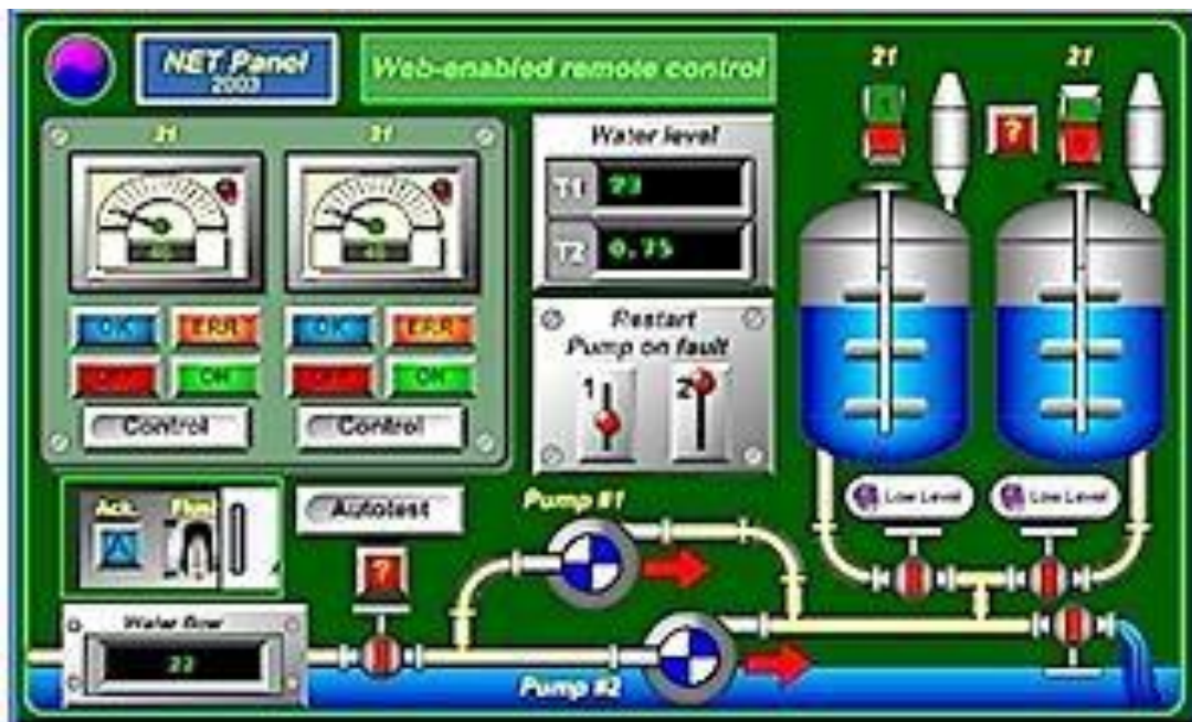
Figure 8: Example SCADA screen including meter and instrument readings. A historian records these readings on regular intervals. This data helps with performance evaluations and process troubleshooting.
