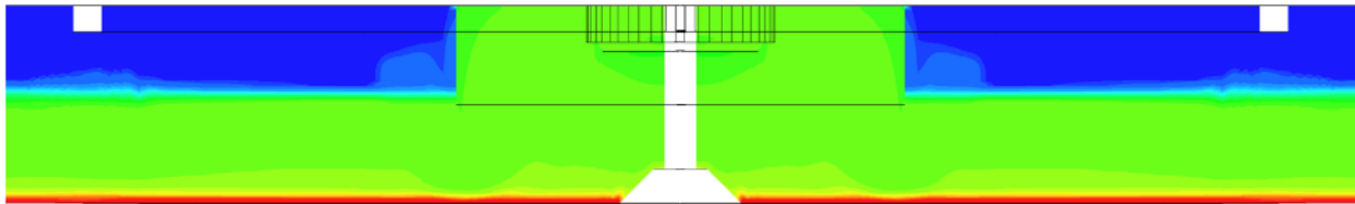
Figure 10: CFD model results for solids concentration of a secondary clarifier. Colors are as follows: dark blue is 10 mg/L, light blue is 1,000 mg/L, green is 3,000 mg/L, and red is 6,000 mg/L.
