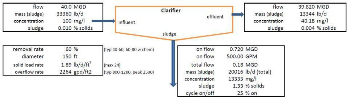
Figure 9: Example mass balance for a clarifier at peak flow. Note the mass of sludge entering the clarifier (33,360 lb/d influent) equals the mass leaving the clarifier (13,344 lb/d effluent plus 20,016 lb/d sludge).
