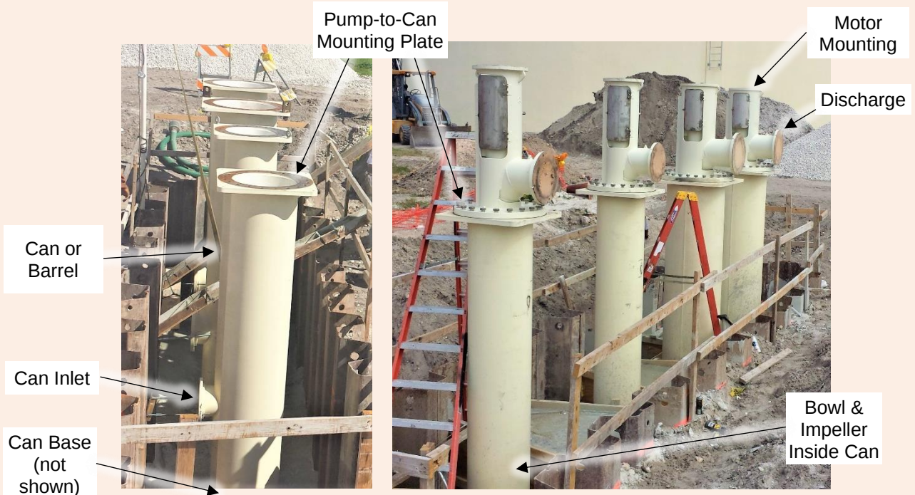
Figure 8: Four vertical can pumps (a.k.a. barrel pumps) prior to encasement in concrete. Left: Cans installed without VS1 pumps. Inlet manifold piping also needs to be installed. Right: After VS1 pumps set into the cans and bolted to the mounting plates.
