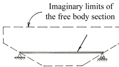
Load Diagram
