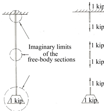
Load Diagram
