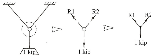
Internal Free-Body Diagram
