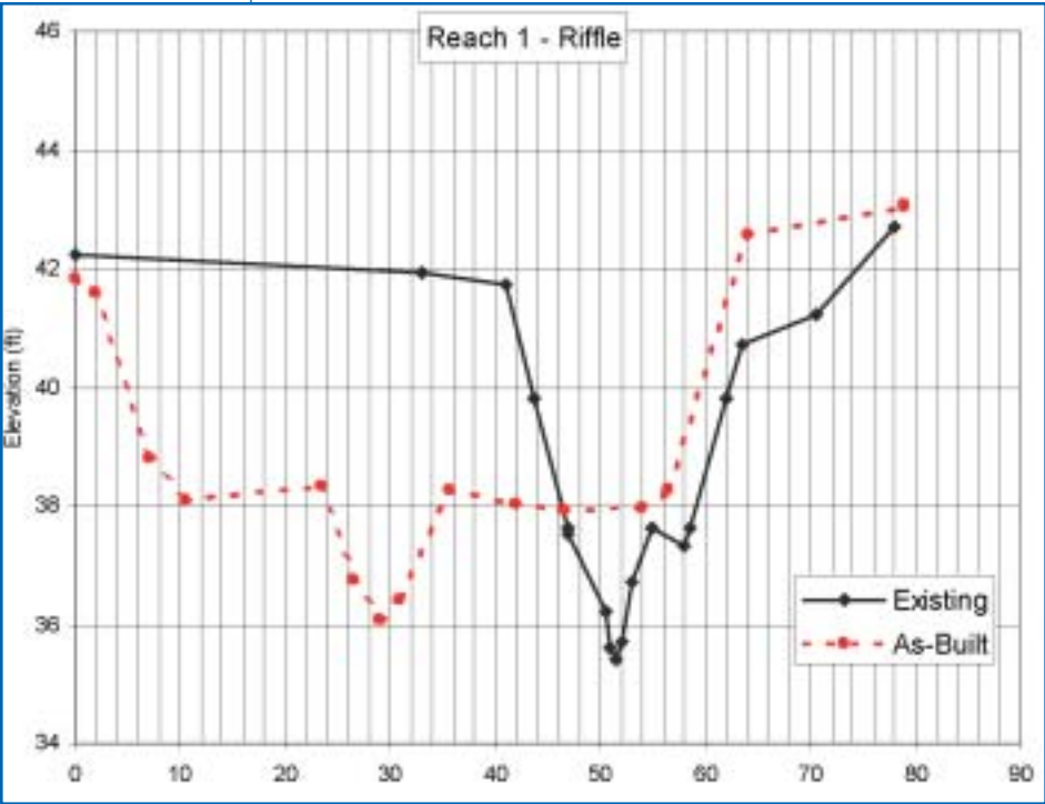
Figure 5.8 Cross-section survey of Pine Valley Golf Course restoration project
