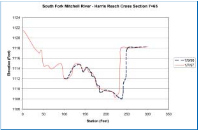
Figure 3.10 Permanent cross-section monitoring results
