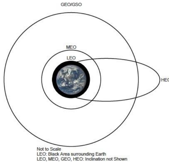
Figure 3: Earth Orbits
