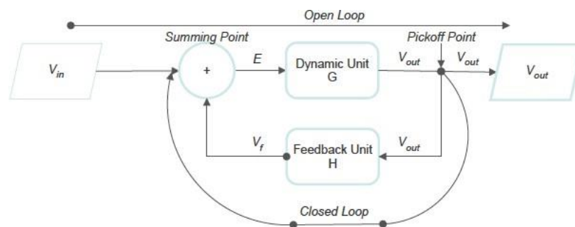
Figure 17: Feedback System
