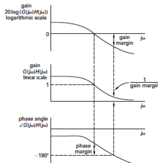
Figure 18: Phase and Gain Margin
