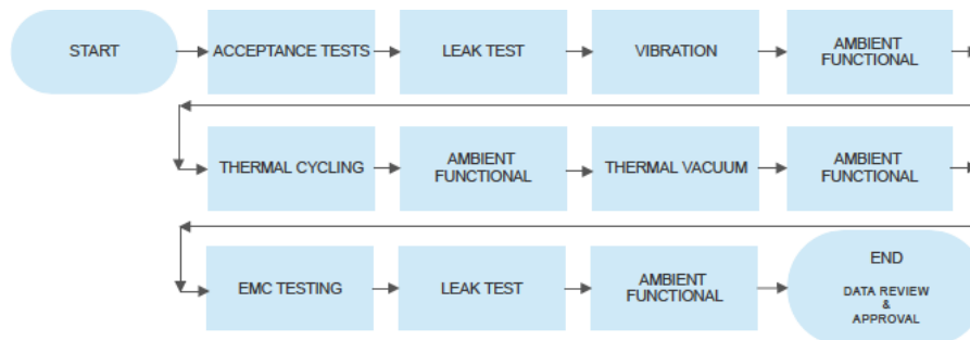
Figure 19: Qualification Testing Sequence Example
