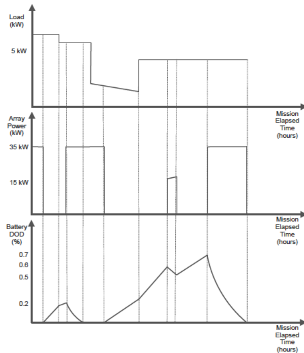
Figure 11: Operational Load Profile--Notional
