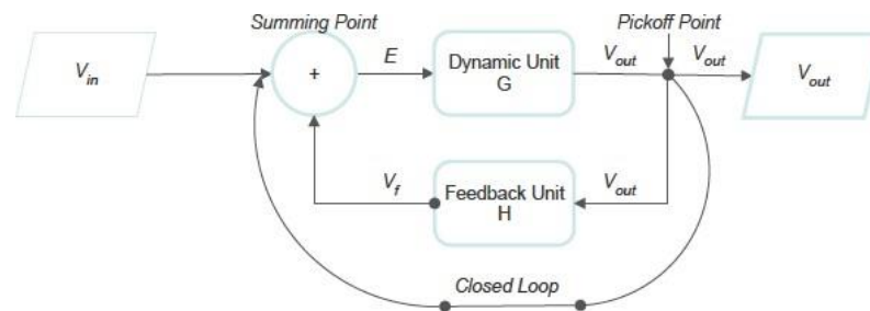
Fig. 10: Regulated System—Closed Loop
