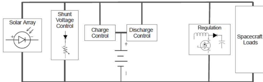
Figure 6: Functional Block Diagram of Typical EPS
