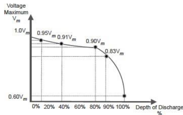
Figure 8: Lithium-Ion Battery Voltage vs Depth-of-Discharge
