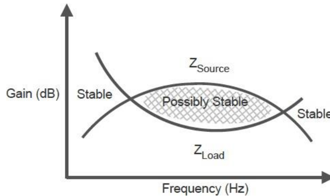
Figure 16: Source and Load Stability
