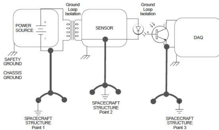
Figure 14(b): Multi-Point Ground Scheme
