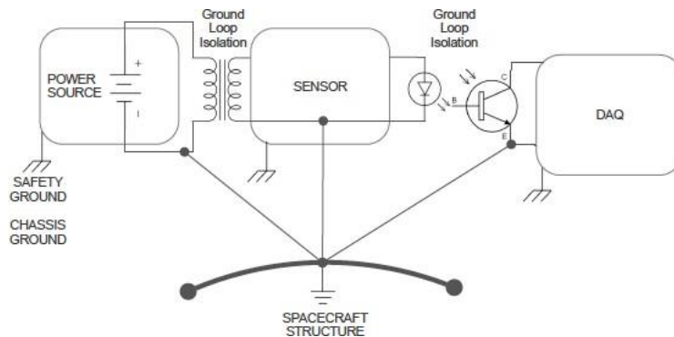
Figure 14(a): Single-Point Ground Scheme
