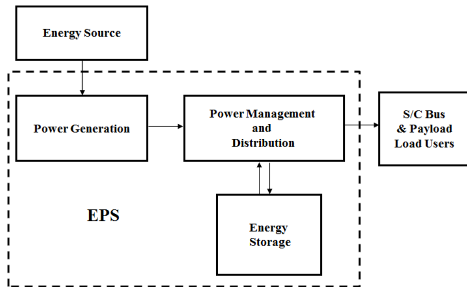
Figure 2: Earth-Orbiting Spacecraft EPS Functional Block Diagram
