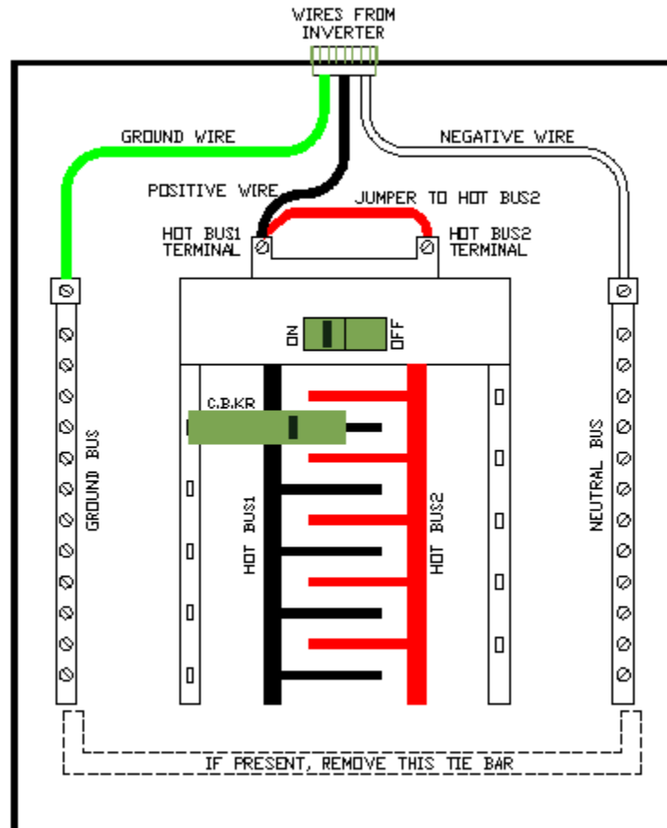
Circuit Breaker Box wiring – Note the Breaker Box may or may not have a main disconnect switch
