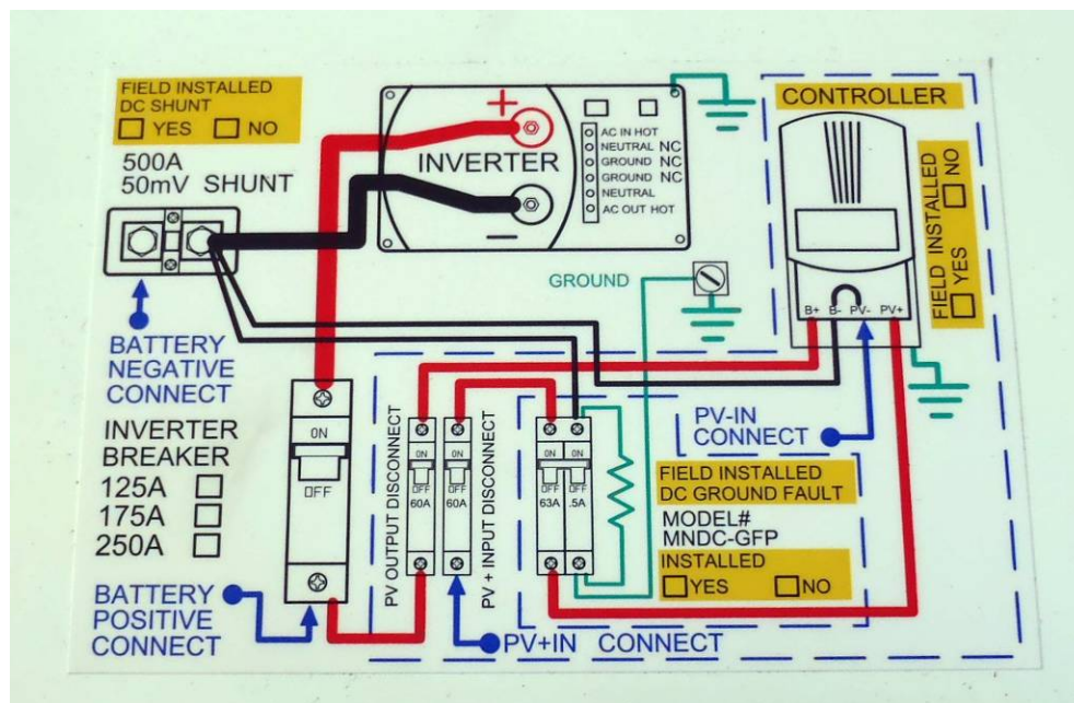
Electrical Disconnect Box wiring diagram provided by the manufacturer
