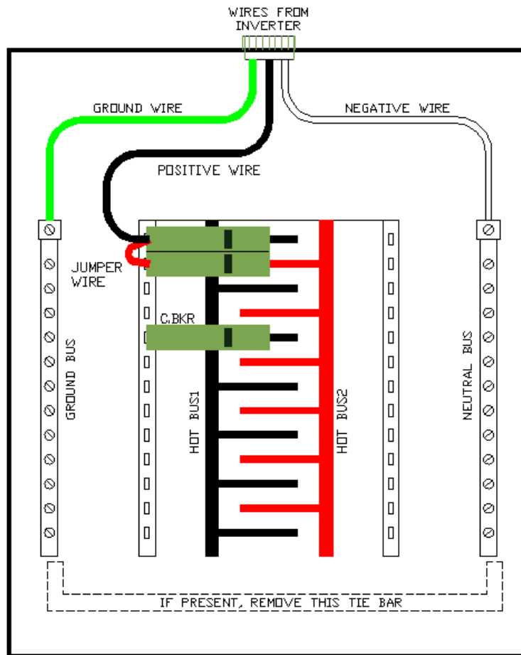
Circuit Breaker Box wiring using circuit breakers to feed both Hot Bus bars
