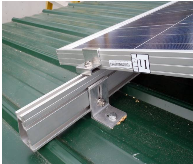
Terminal end clamp
