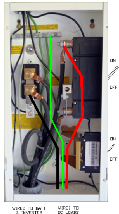
Wiring diagram of the Electrical Disconnect Box for the installation of a DC Load or Circuit Breaker Box
