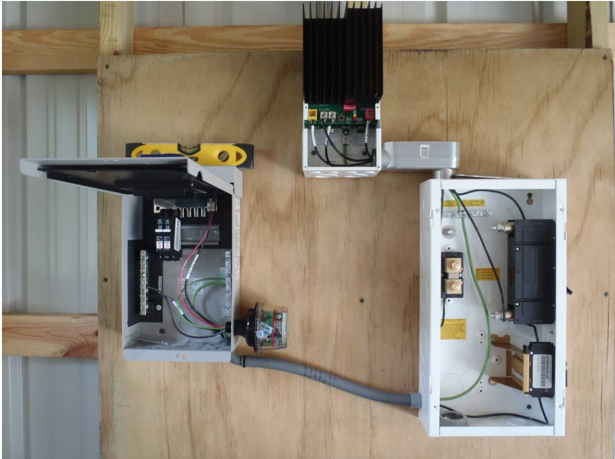
Initial configuration of PV Combiner box, Electrical Disconnect Box, and Charge Controller. The Monitor Meter attached directly to the Charge Controller in this installation.
