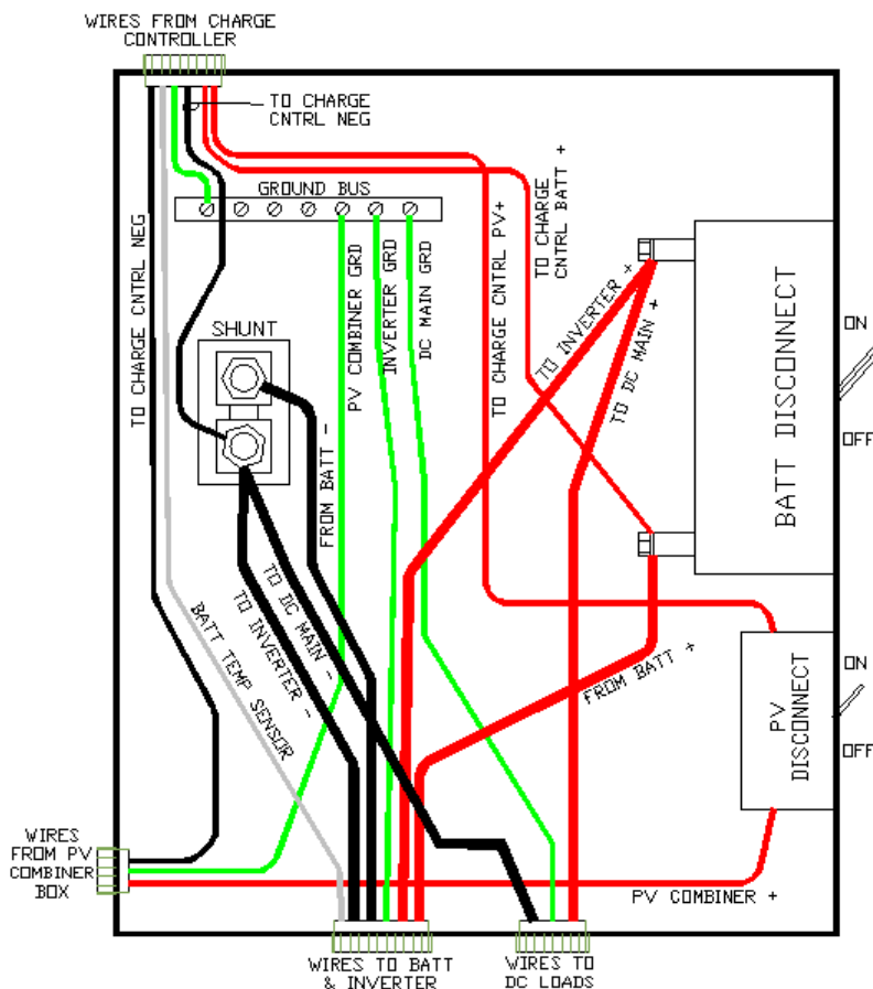
Wiring diagram of the Electrical Disconnect Box for the installation of a DC Load or Circuit Breaker Box
