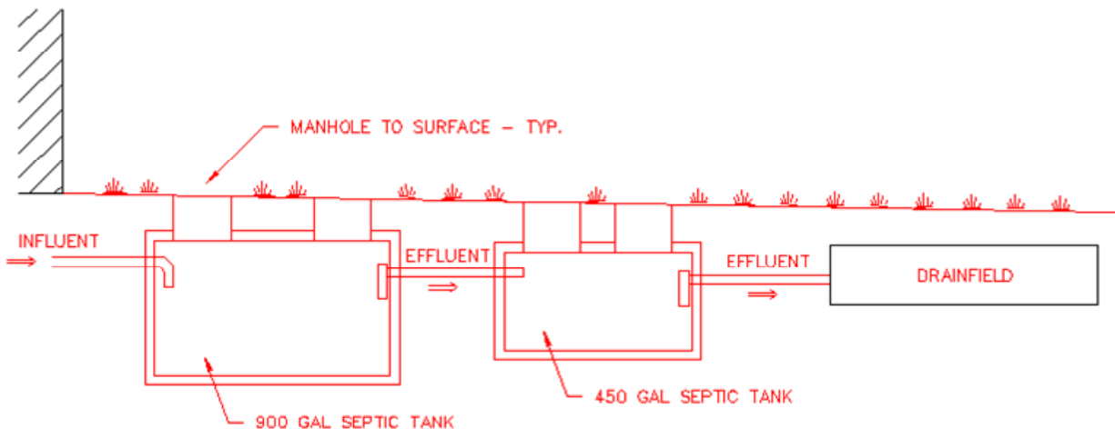
Gravity Septic System Layout
