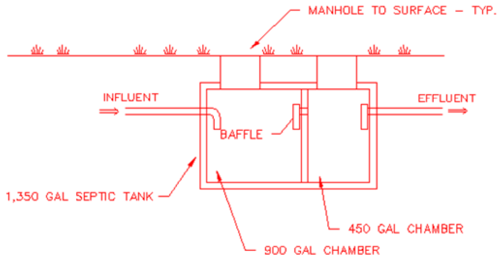
Septic Tank with Baffle
