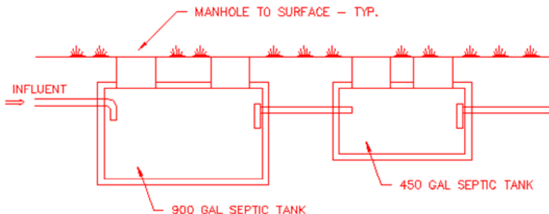
Septic Tank in Series
