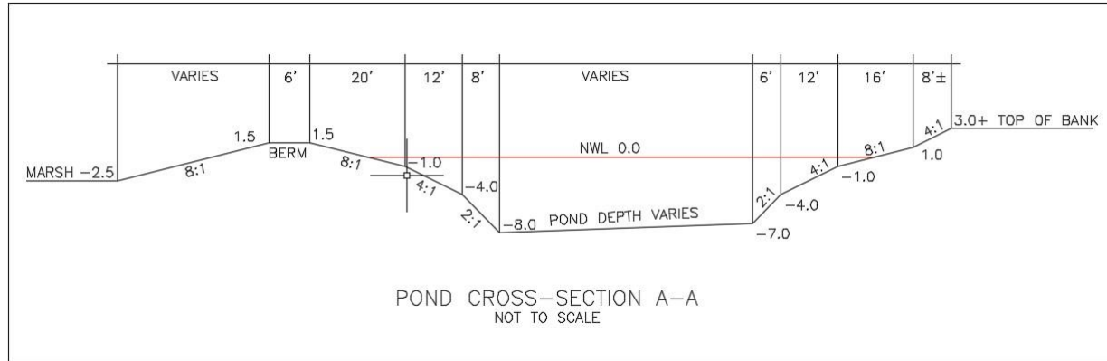
Figure 14 - Cross-section of Pond Side Slopes
