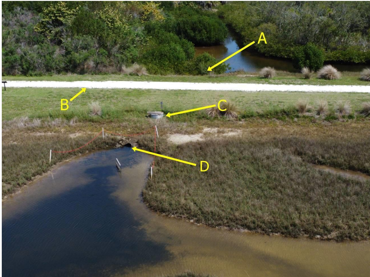
Figure 4 – Tidal Creek connection (A), Isolation Berm (B), Water Control Structure (C), Tidal Marsh connection (D)
