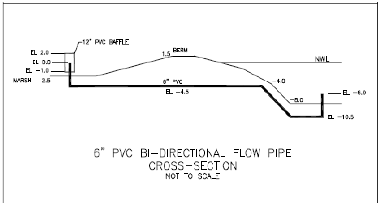
Figure 9 – Bi-directional flow pipes detail
