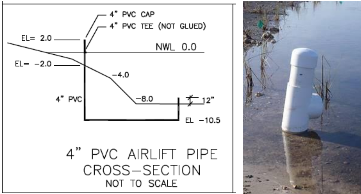
Figure 11 – Tidal Pond Air Lifts
