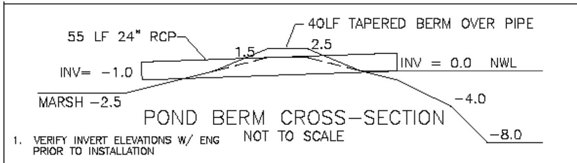
Figure 7 – Pond cross-section at culvert crossing
