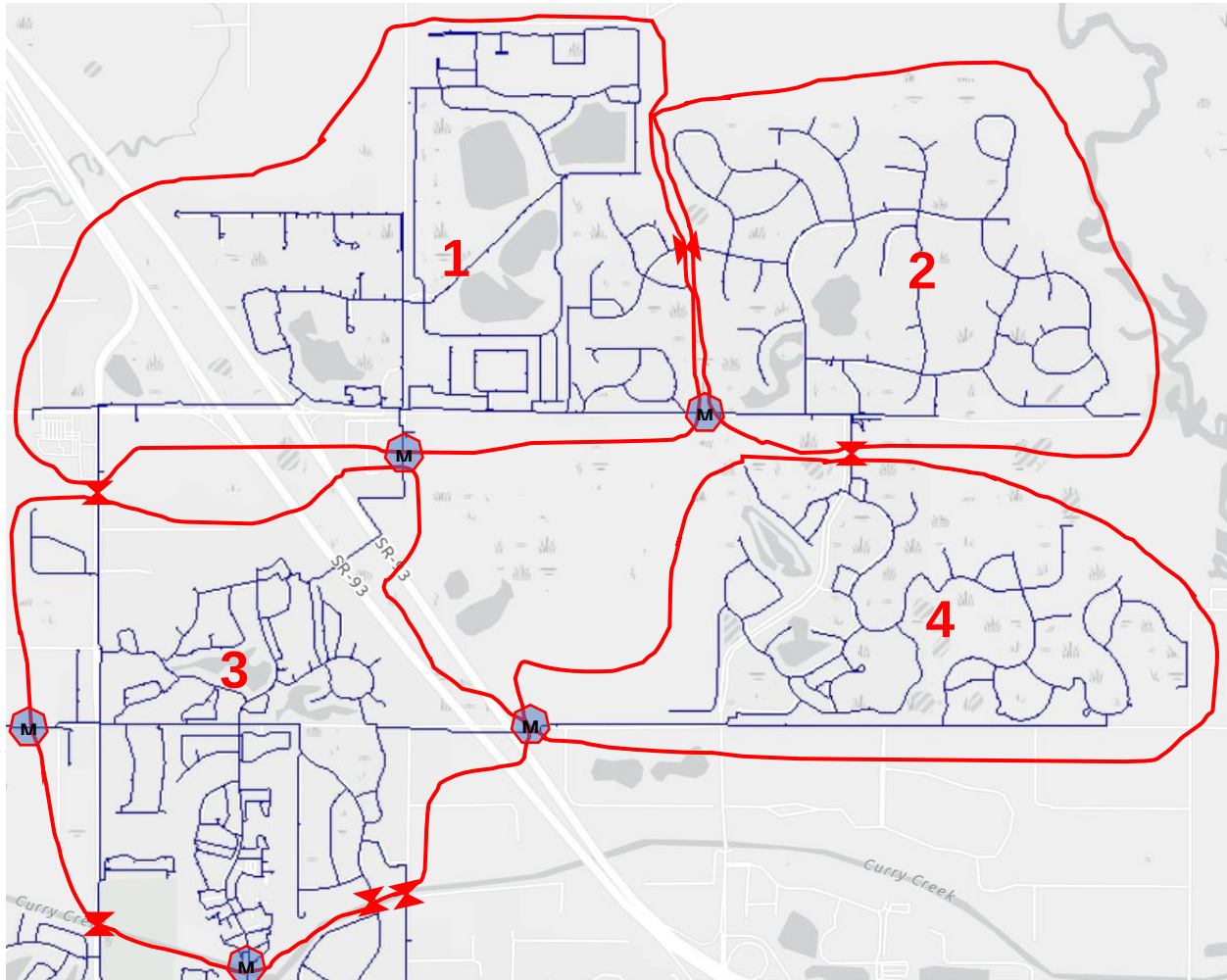
Figure 16: GIS screenshot with 4 DMAs created with 5 zone meters and 6 closed valves. Closing valves is more economical than using all flow meters.
