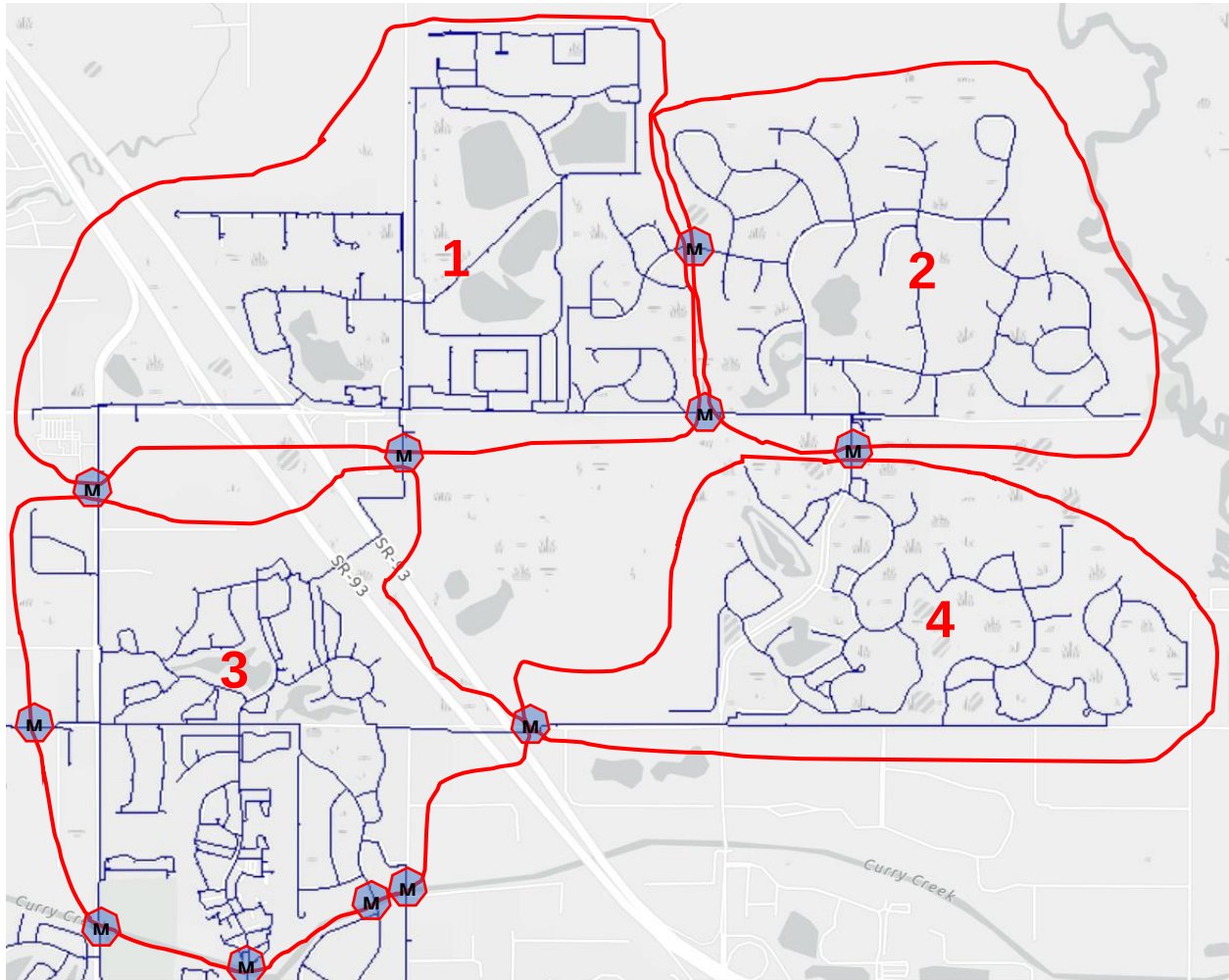
Figure 15: GIS screenshot with 4 DMAs created with 11 zone meters.
