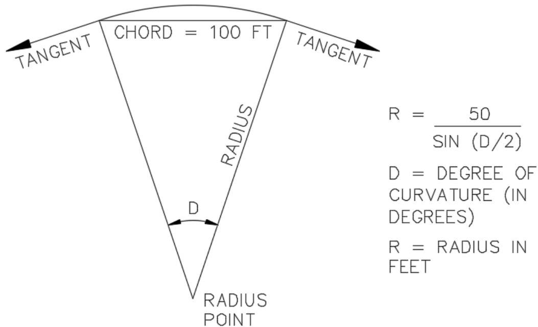
Figure 4 - Railway curve definition
