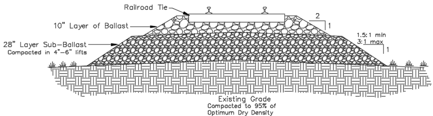
Figure 10 - Example for Heavy-Duty Track Cross-section
