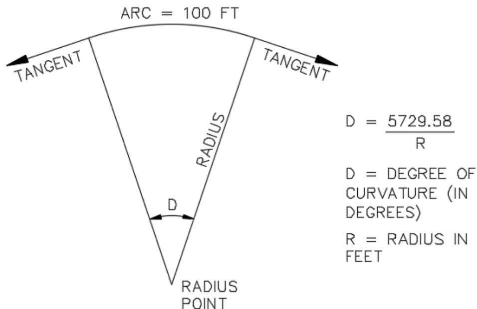
Figure 3 - Highway curve definition
