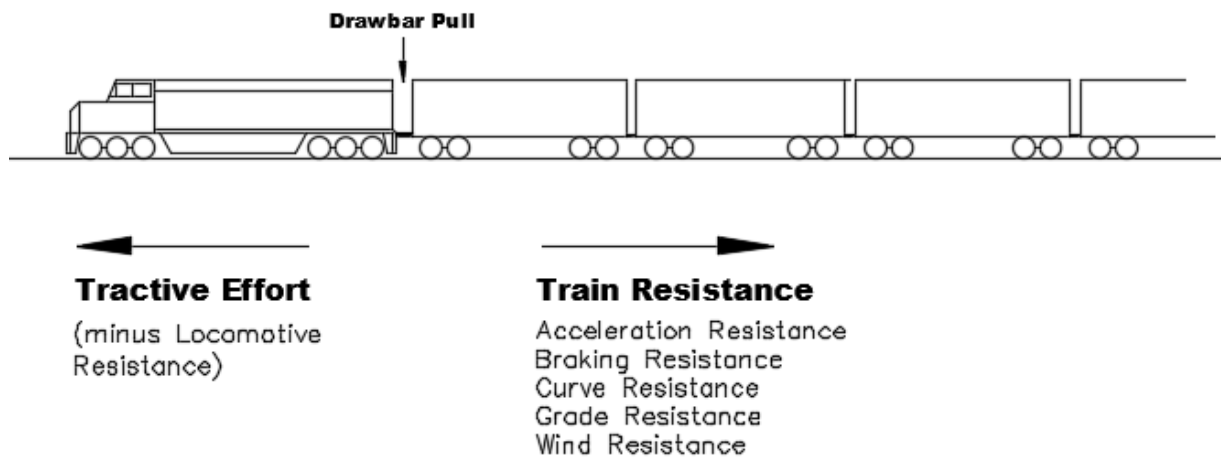
Figure 2 - Railroad forces
