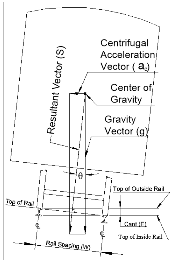
Figure 3 - The combined effects of gravity and centrifugal force
