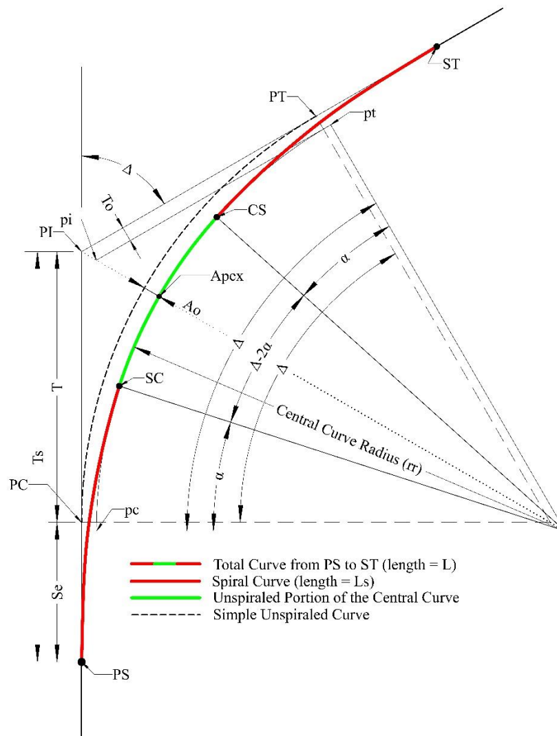
Figure 14 – The Spiral Curve Legend
