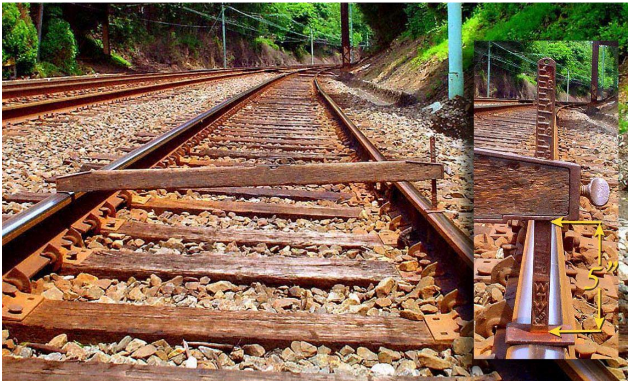
Figure 2 - A spirit level used to measure track superelevation (showing 5")
