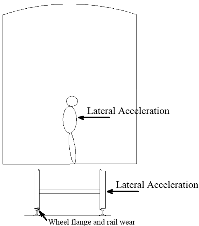
Figure 4 - Cant Deficiency introduces lateral Acceleration.
