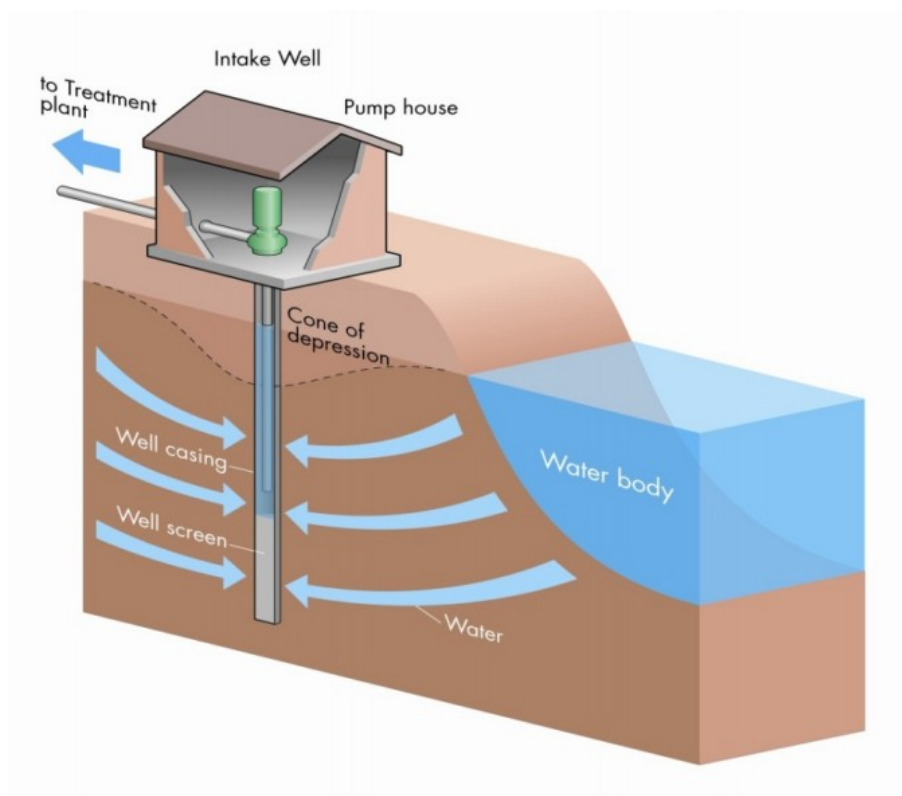
Figure 16: Example of a beach intake well
