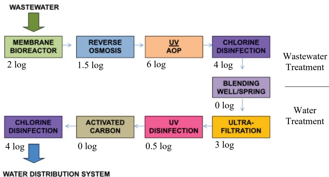
Figure 18: Example flow diagram for a direct potable reuse system, with the wastewater treatment processes at the top and water treatment processes at the bottom. AOP stands for Advanced Oxidation Process. The log removal of viruses is stated for each process, with a total of 21 log removal.
