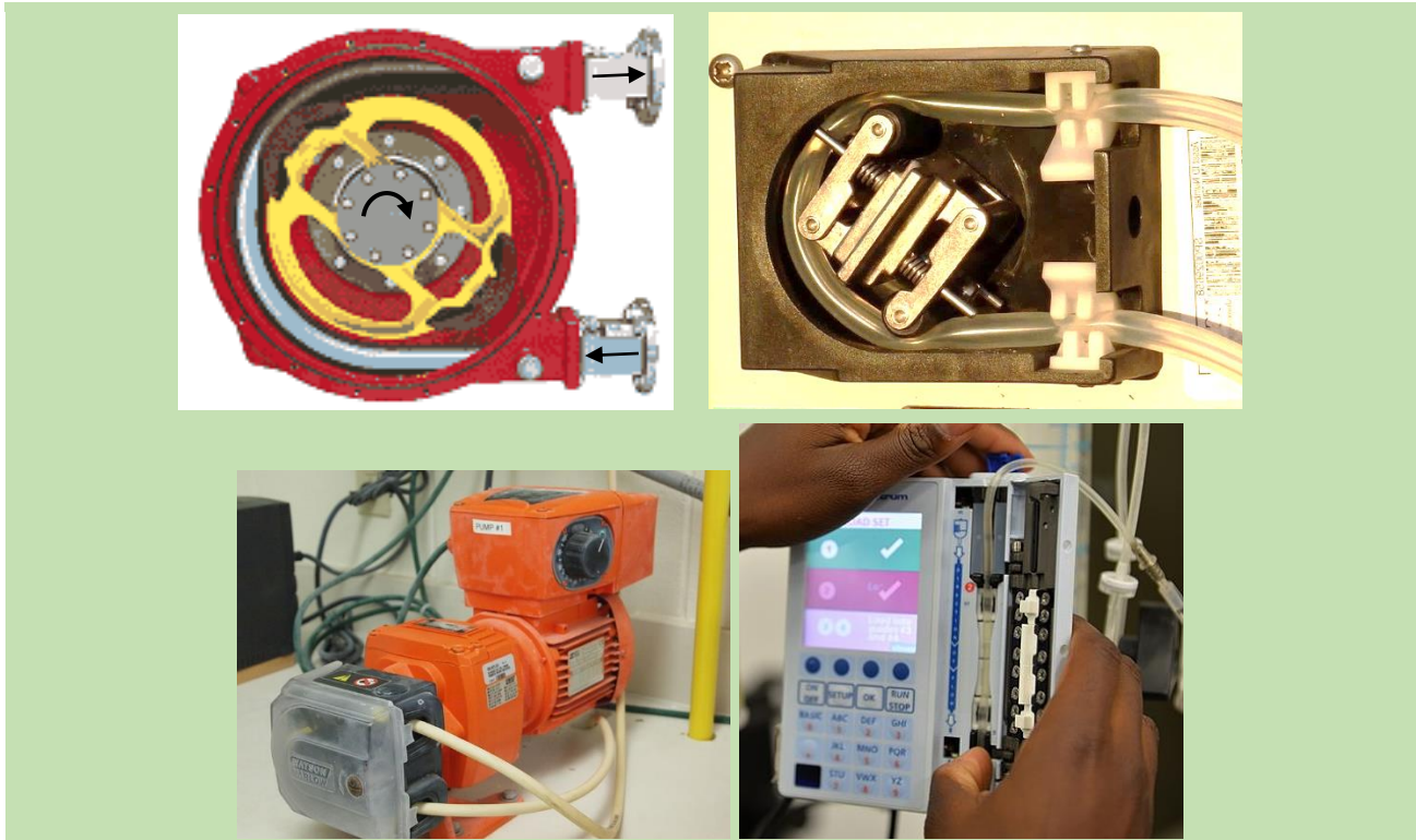
Figure 9: Top left: Hose pump internals with two shoes in black. Top right: Tube pump internals with two rollers squeezing the clear tubing. Bottom left: Example of a chemical metering tube pump with a speed control knob. Bottom right: Linear IV infusion pump for injecting fluids into a patient.
