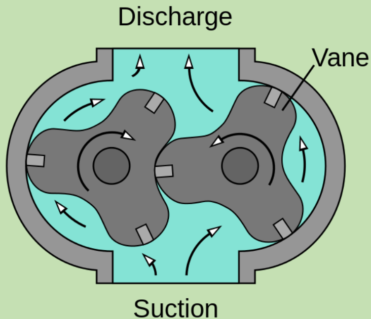
Figure 13: Section of a lobe pump with labels and flow direction arrows.
