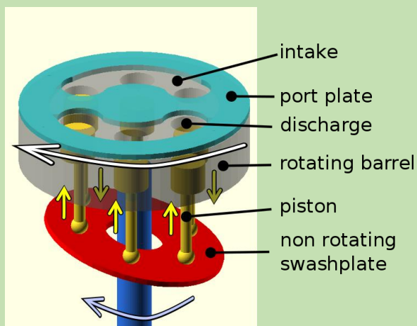
Figure 11: On the left, schematic of an axial pump. Three pistons move up (discharge) and three pistons move down (intake cycle). On the right, an example of an axial pump with the casing partially removed.
