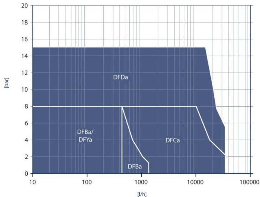
Figure 23: Example chart of capacity and pressure ranges for various diaphragm pump models. Note that 1 liter per hour (l/h) = 0.2642 gph and 1 bar = 14.5 psi.
