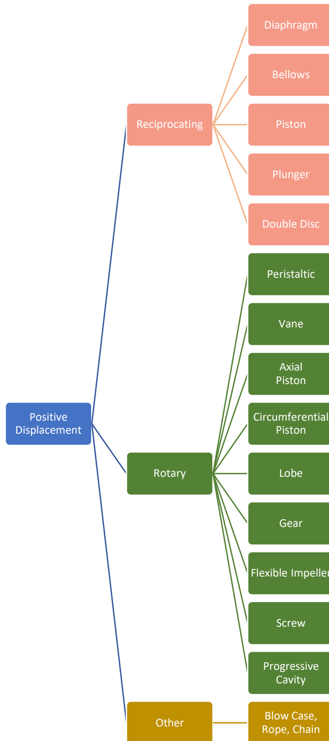
Figure 2: Chart of Positive Displacement Pump Types
