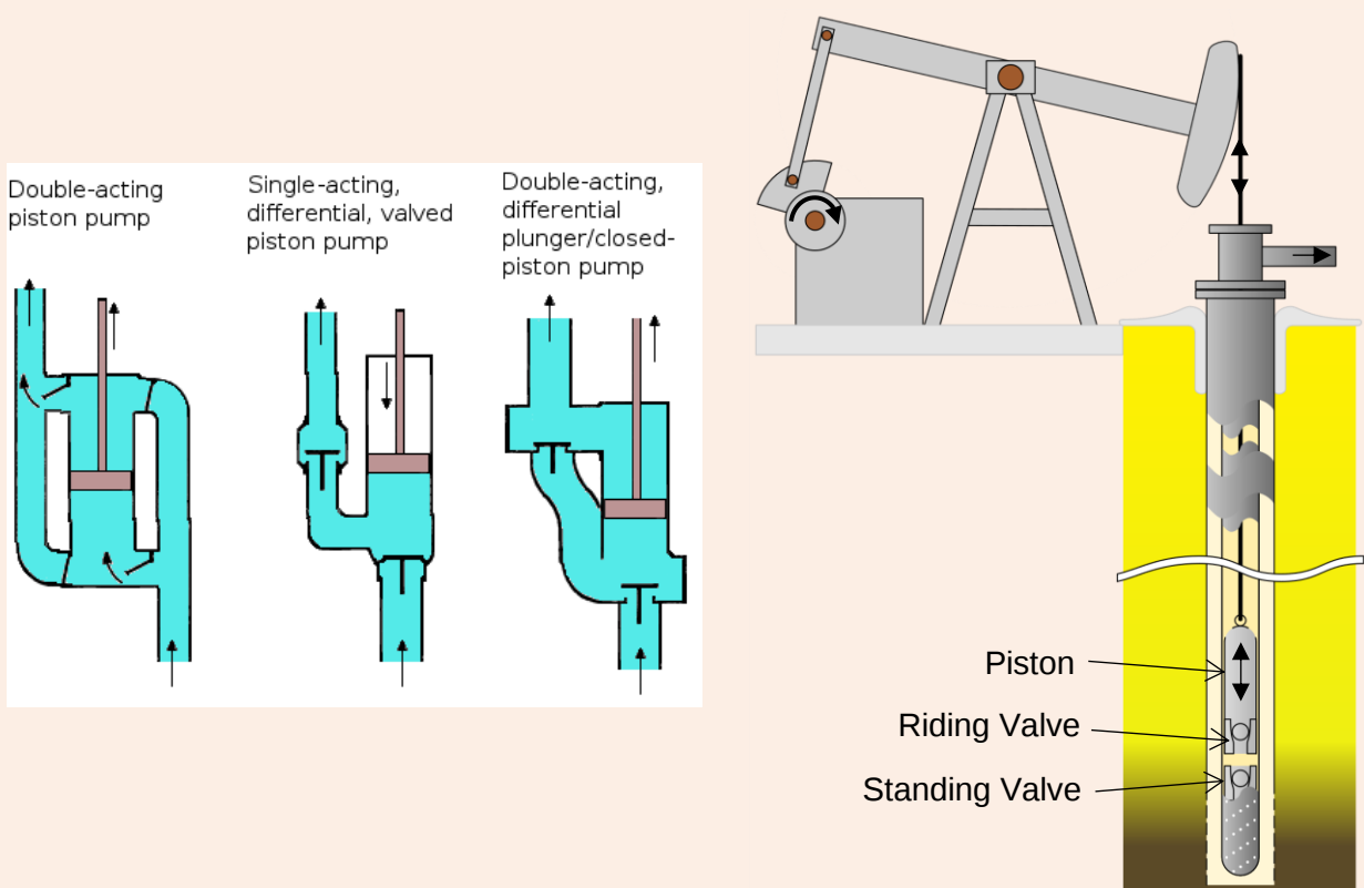
Figure 6: On the left, three common arrangements for piston pumps. On the right, a pumpjack for an oil well, which is a unique piston pump arrangement.
