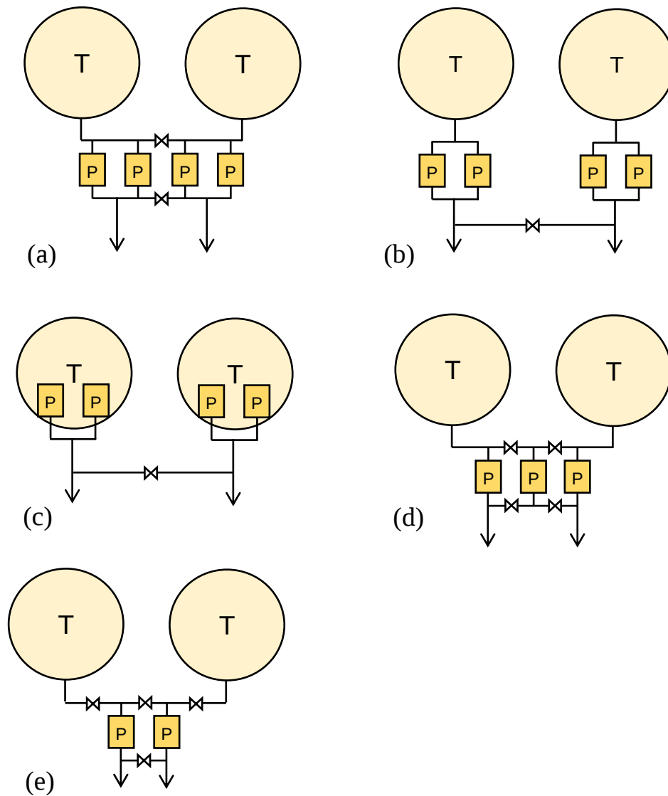
Figure 18: Alternative tank (T) and pump (P) arrangements to provide for redundancy of tanks, pumps, and piping. For (c), the pumps are mounted on top of the tanks.
