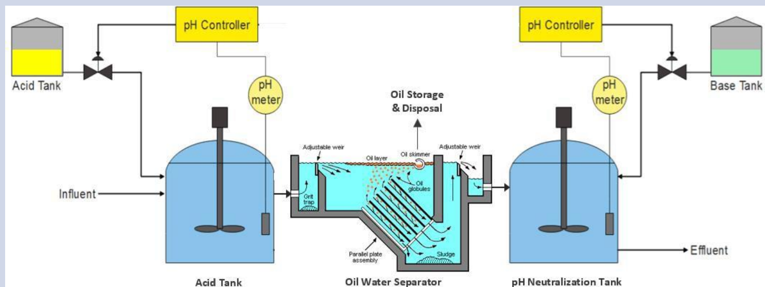
Figure 15: pH Adjustment system starting with acid to lower pH, oil removal, then base to raise pH back to neutral.
