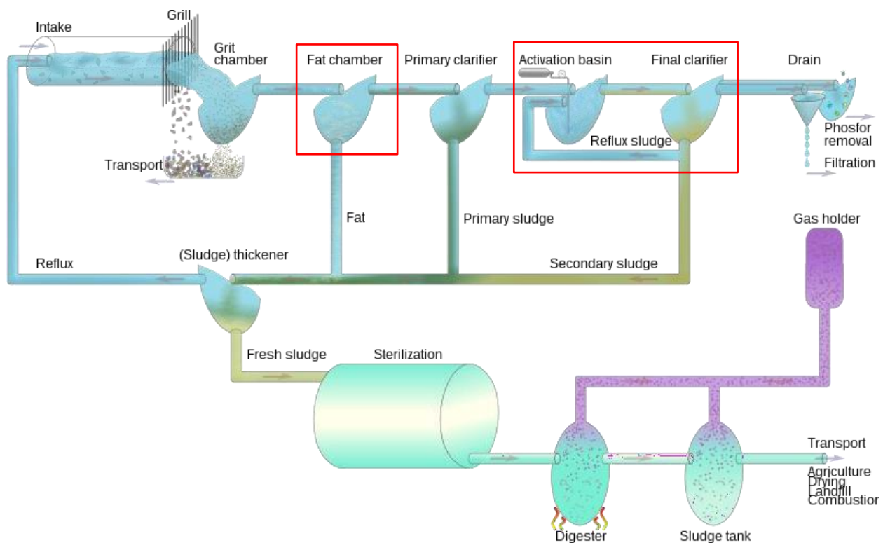
Figure 4: A WWTP flow diagram with processes that remove O&G highlighted red. The activated basin and final clarifier together form an activated sludge biological treatment process that breaks down various forms of O&G into secondary sludge.
