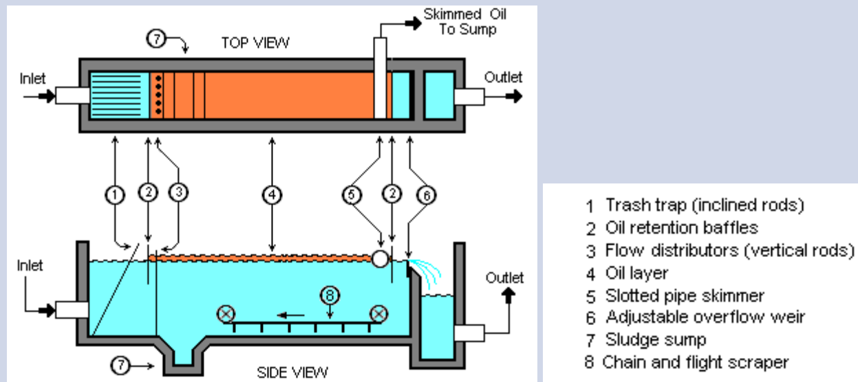
Figure 14: Typical API separator with labels. The scraper can collect O&G at the surface and sludge at the floor.
