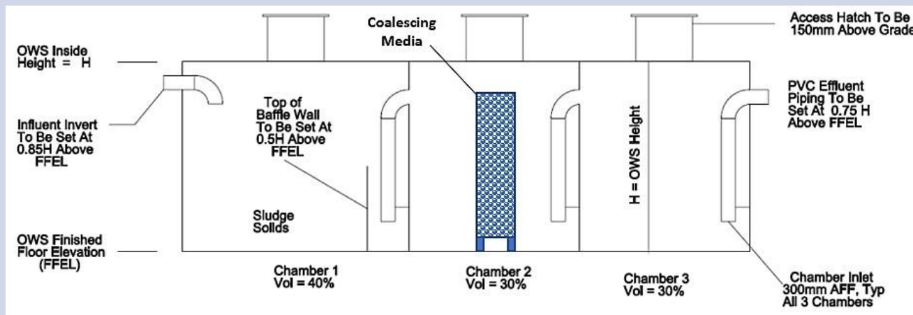
Figure 13: Oil water separator design with three chambers and coalescing media.
