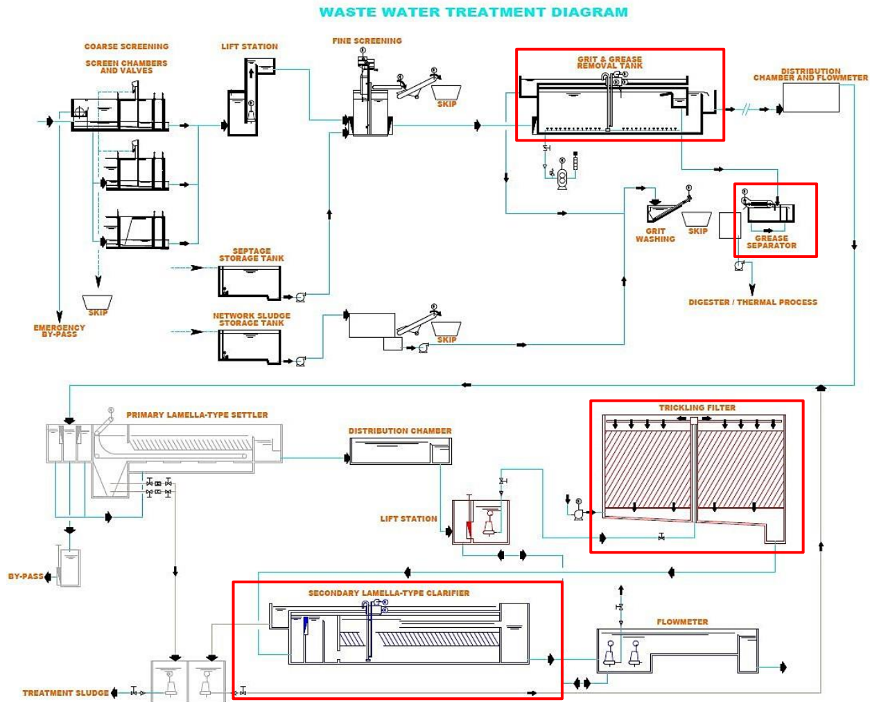
Figure 5: A WWTP flow diagram with processes that remove O&G highlighted red. The trickling filter and clarifier together form a biological treatment process that breaks down various forms of O&G into sludge that is settled and removed.
