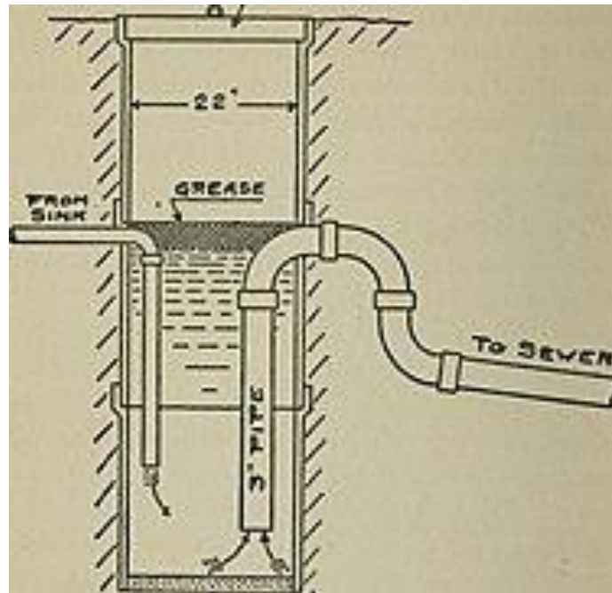
Figure 1: Example of buried grease trap design published in “The Farmer His Own Builder” in 1918.
