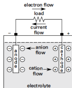
Figure 4: Battery Standard Terminology
