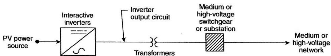
Figure 14: Large-Scale PV Electric Supply Station
