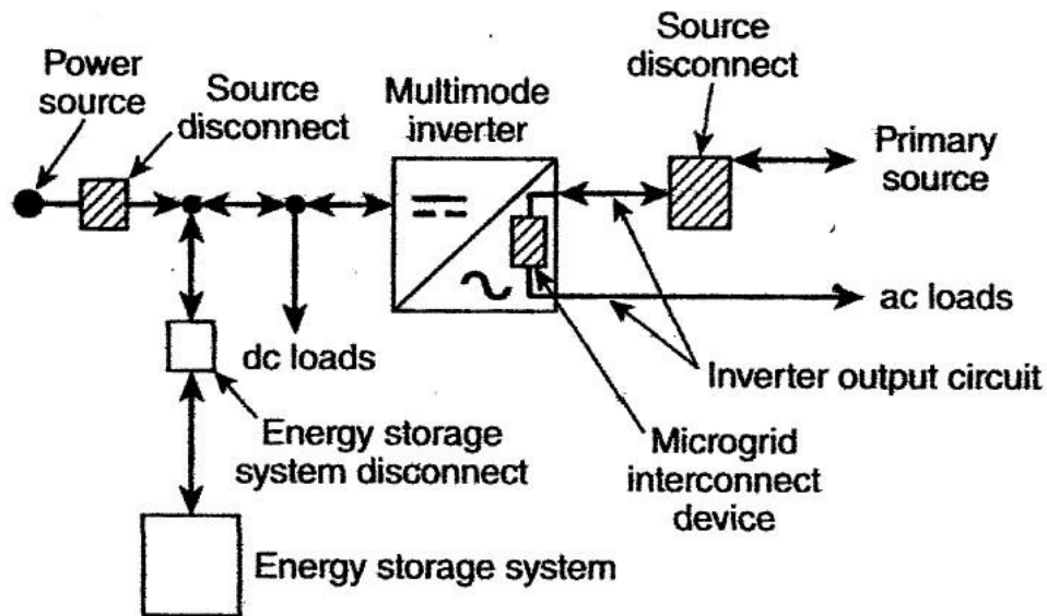
Figure 15: DC Interconnected System
