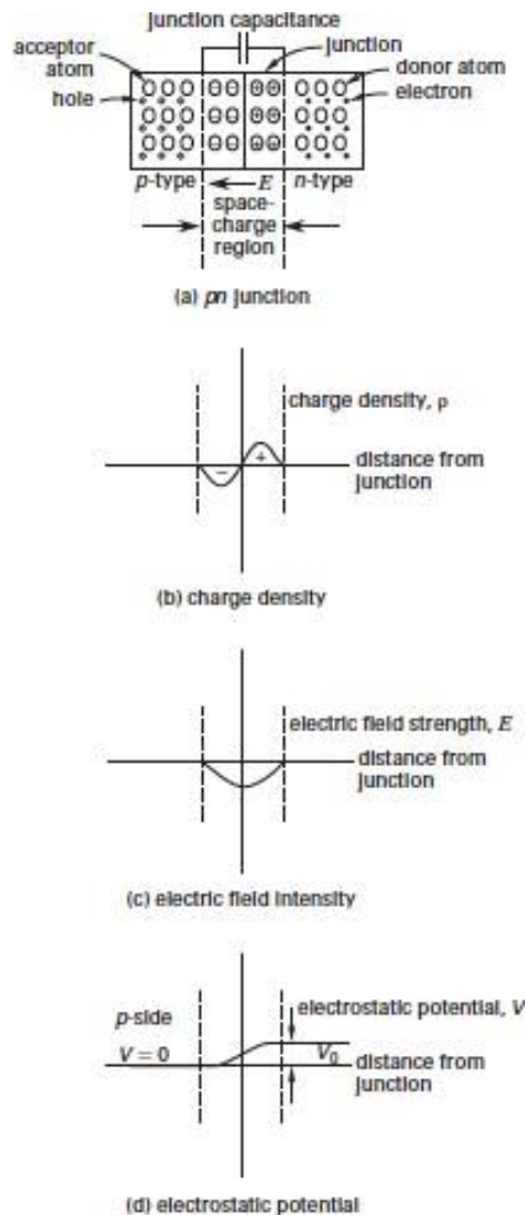
Figure 9: Junction Characteristics of a pn Junction
