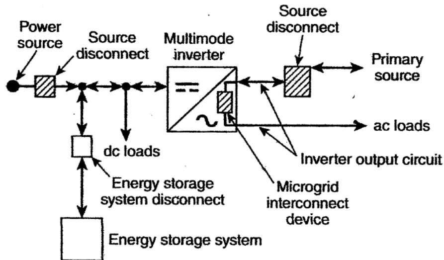
Figure 7: DC Interconnected System
