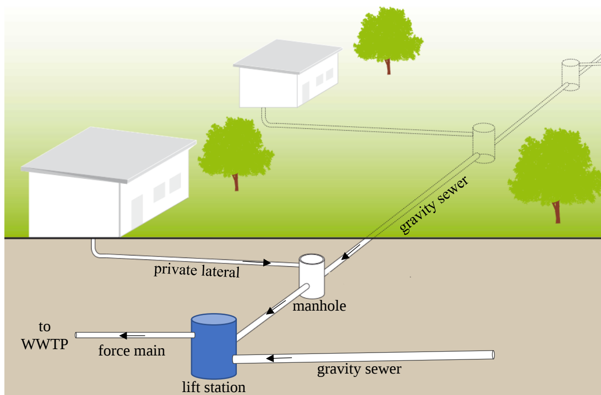
Figure 1: Schematic of a wastewater collection system with a lift station in blue.
