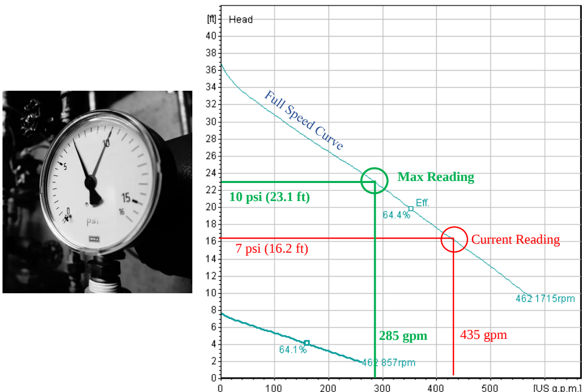
Figure 4: Left: A force main pressure reading of 7 psi (16.2 ft) and a max pointer reading of 10 psi (23.1 ft). Right: Pump curve with corresponding operating points. These pressure readings also help define the force main pressure range, which is needed later for producing the system curve.
