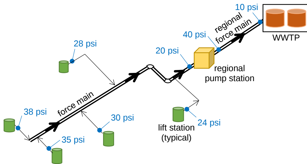
Figure 3: Force main schematic showing design pressures at each facility.
