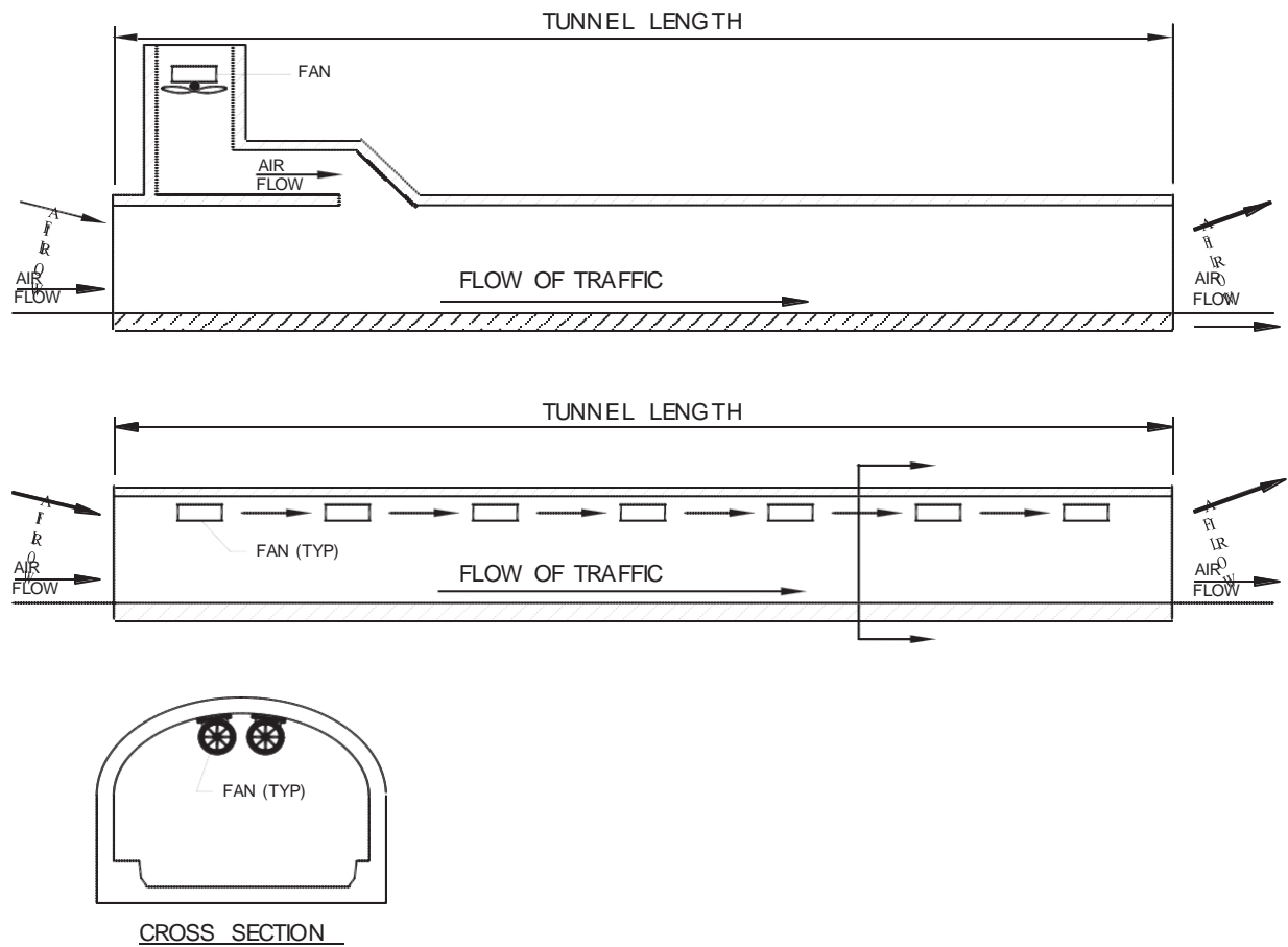
Figure 2.14 – Longitudinal Ventilation
