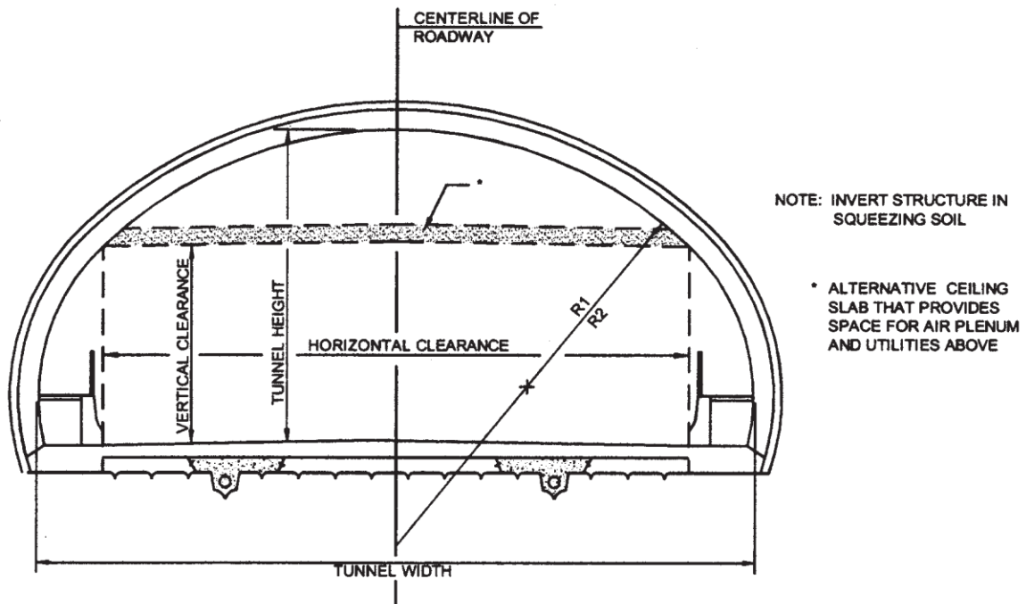
Figure 2.4 – Oval/egg tunnel with three traffic lanes and two safety walks. Also shown is alternative ceiling slab.
