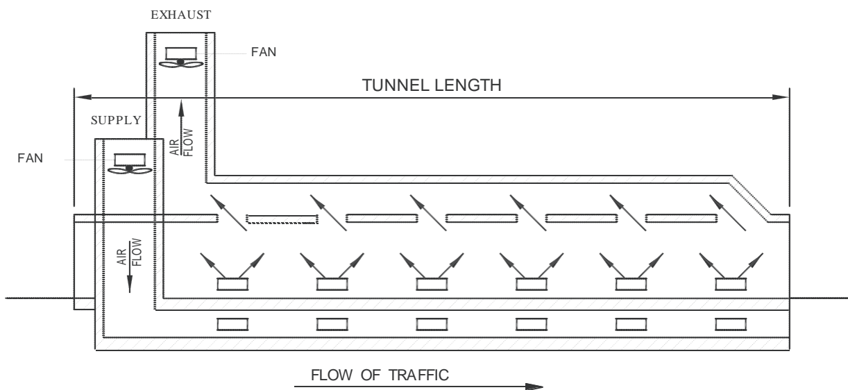
Figure 2.16 – Full-Transverse Ventilation
