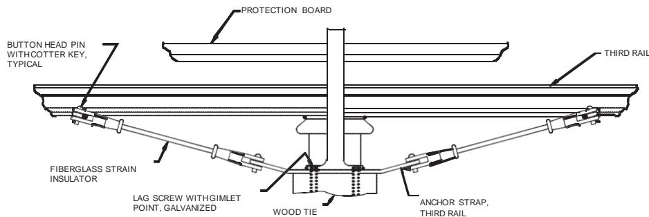
Figure 2.20 – Typical Third Rail Insulated Anchor Arm
