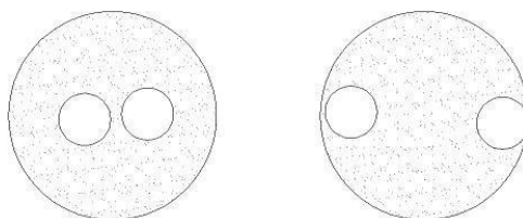
Figure 17 Cross-sectional Drawing of 1 1/4" loop pipes in a 6" borehole.
