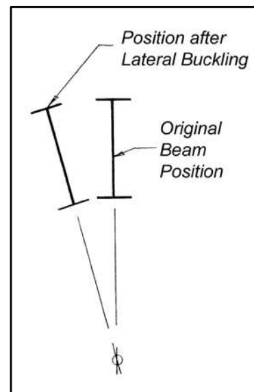
Figure 16 - Lateral buckling of top flange
