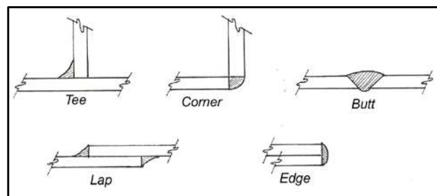
Figure 6 – Weld Joints
