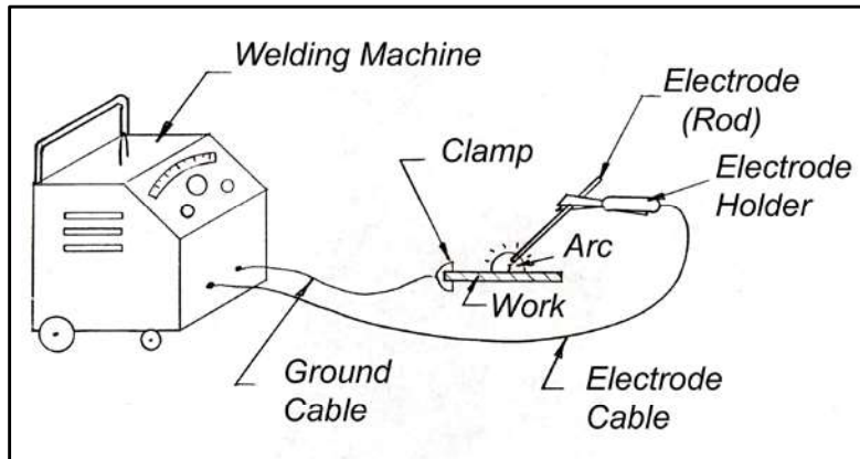
Figure 1 - Depiction of an electric arc welding system
