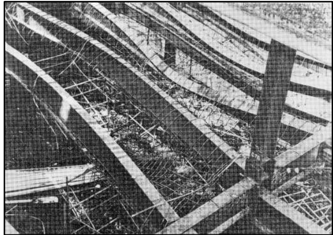
Photo No. 10 - Steel beams after a fire
