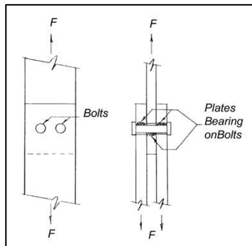
Figure 10 - Bolted Connection - Double Shear
