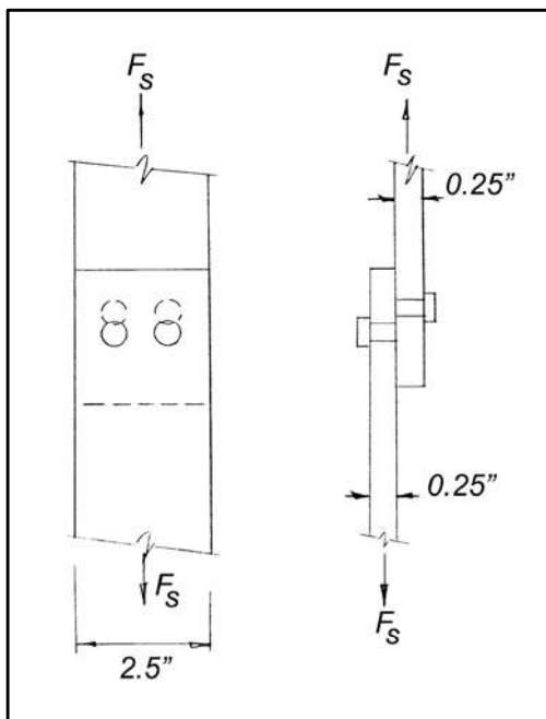
Figure 14 - Shear
