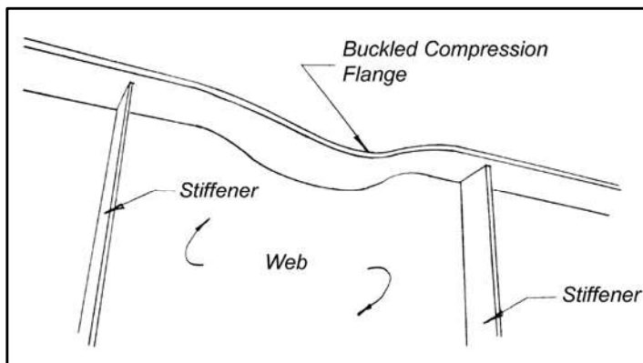
Figure 15 - Instability due to vertical buckling of compression flange
