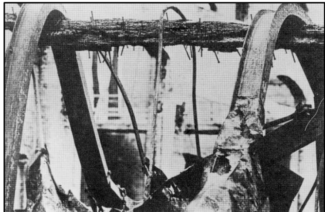
Photo No. 14 - Fire reduced strength of steel to zero
