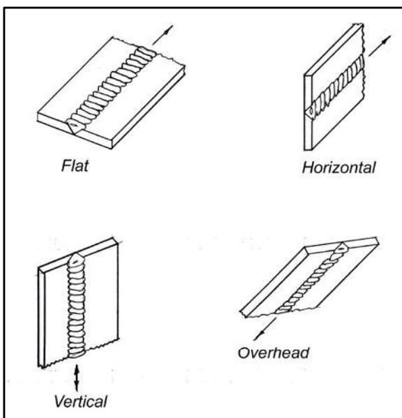
Figure 7 - Weld Positions
