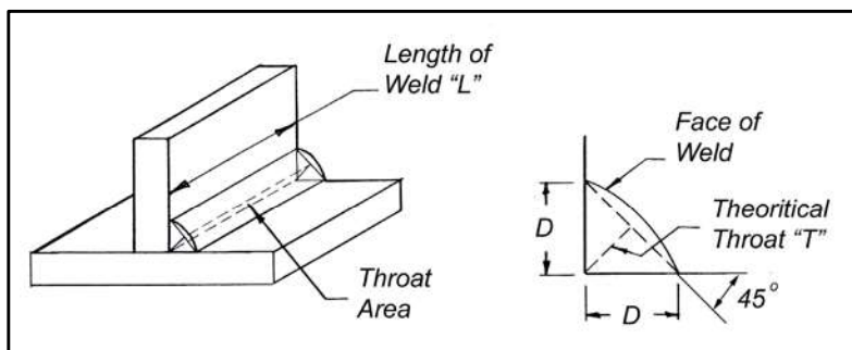
Figure 8 – Area of Throat
