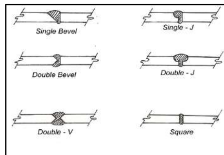
Figure 5- Butt Welds
