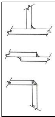
Figure 4 – Fillet Welds
