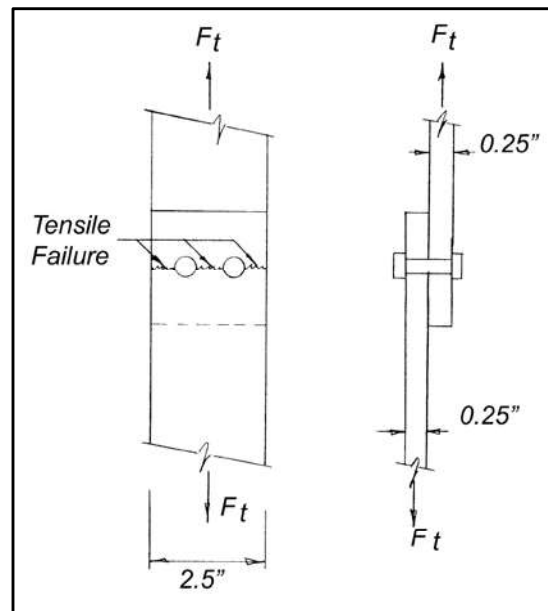
Figure 13 – Tensile failure
