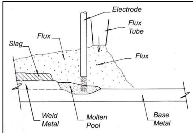
Figure 3 - Submerged arc-welding process
