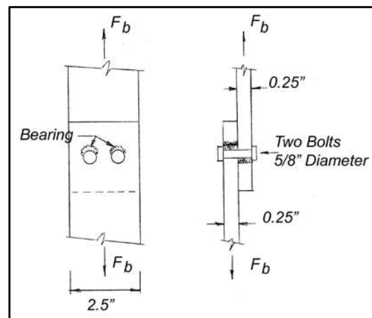
Figure 12 – Bearing failure
