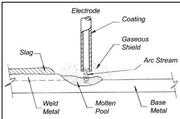
Figure 2 - Shielded arc-welding process
