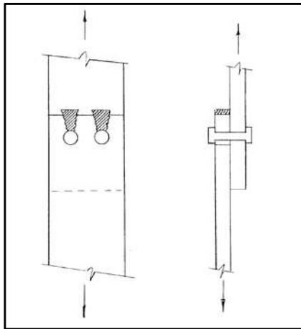
Figure 11 - End tear-out failure
