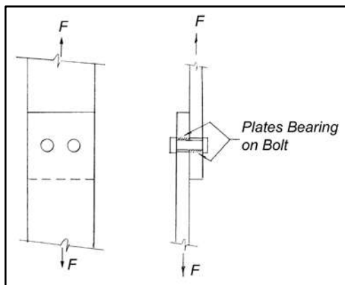
Figure 9 – Bolt Connection-Single Shear
