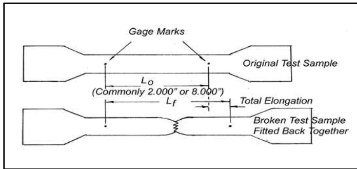
Figure 6 - Illustration of test sample before and after being pulled to failure
