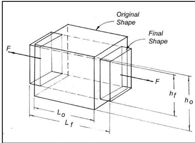
Figure 4 - Illustration of Poisson's ratio for an element in tension
