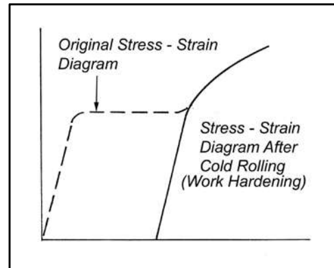
Figure 8 - Effects of cold rolling (work hardening) on the stress-strain diagram for structural carbon steel
