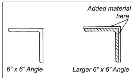
Figure 12 - Angle and additional material for a larger angle of same nominal size
