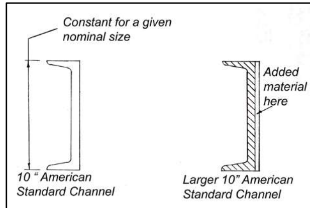
Figure 11 - American Standard Channel and additional material for a larger channel of same nominal size
