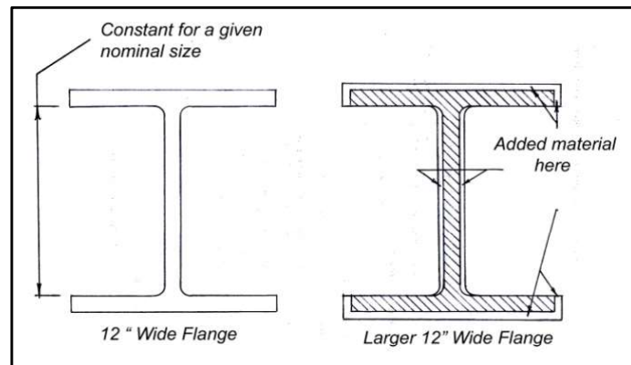
Figure 9 - Wide flange shape and additional material for a larger wide flange of same nominal size
