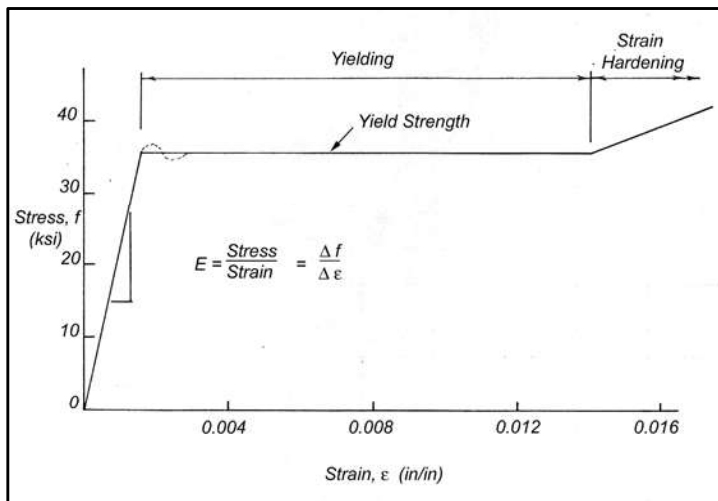
Figure 3 - Portion of a stress - strain diagram for structural carbon steel
