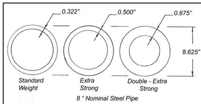
Figure 13 - Illustration of wall thickness for different classification of steel pipe
