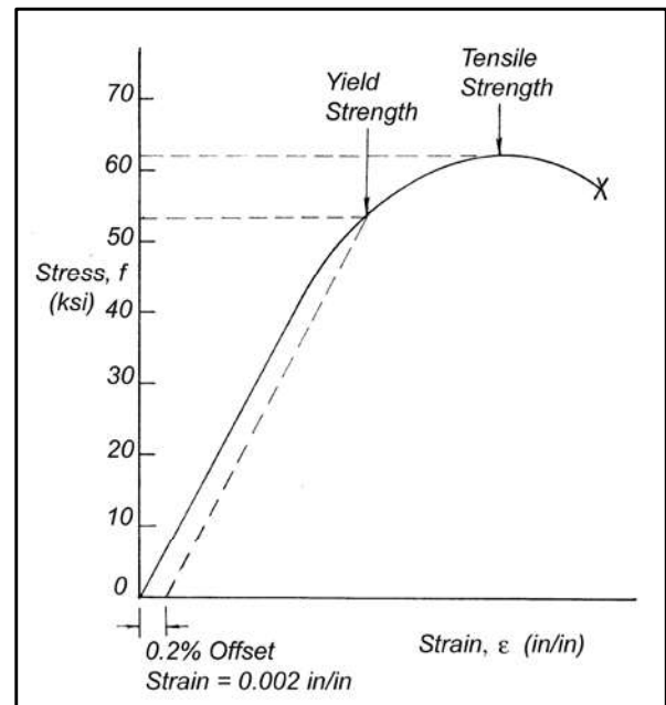
Figure 2 - Typical stress - strain diagram for structural carbon steel without a yield point
