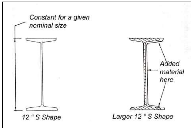
Figure 10 - S Shape and additional material for a larger S Shape of same nominal size
