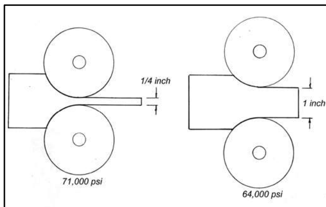
Figure 7 - Effect of rolling on strength of structural carbon steel
