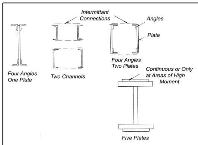
Figure 15 - Various built-up members
