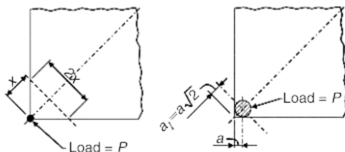
Fig. 6.1—Corner load on slab-on-ground.
