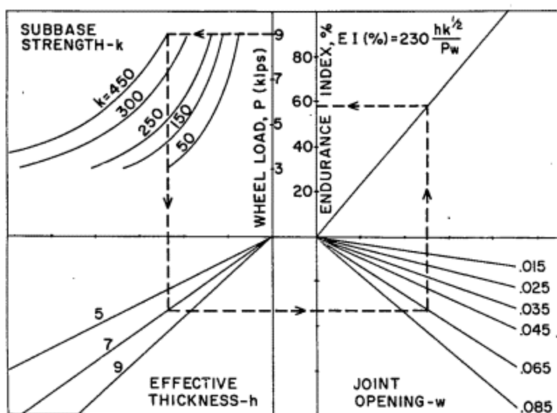
Figure 22. Endurance of joints.
