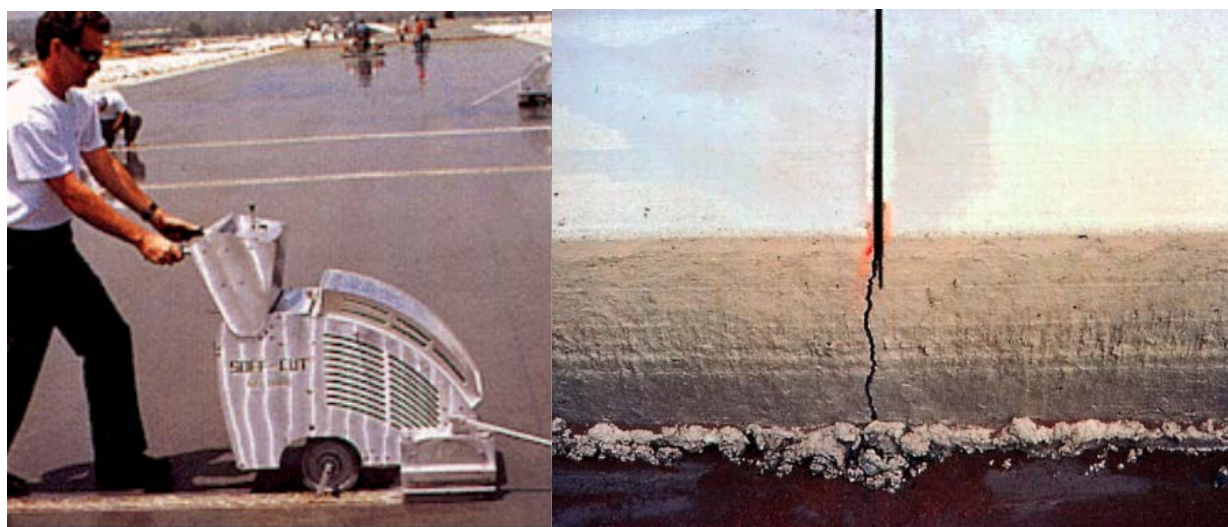
Fig. 32 - Sawcutting new concrete, and joint with crack induced by sawcut (MnDOT)
