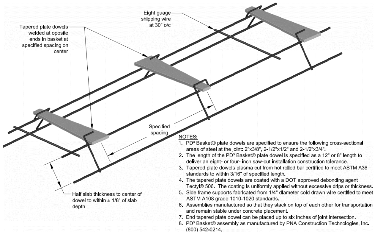
Fig. 43 - Tapered dowels by PNA (PD³ Basket dowels)
