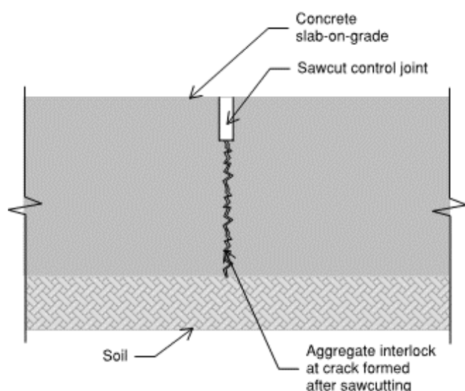
Fig. 34 – Aggregate interlock
