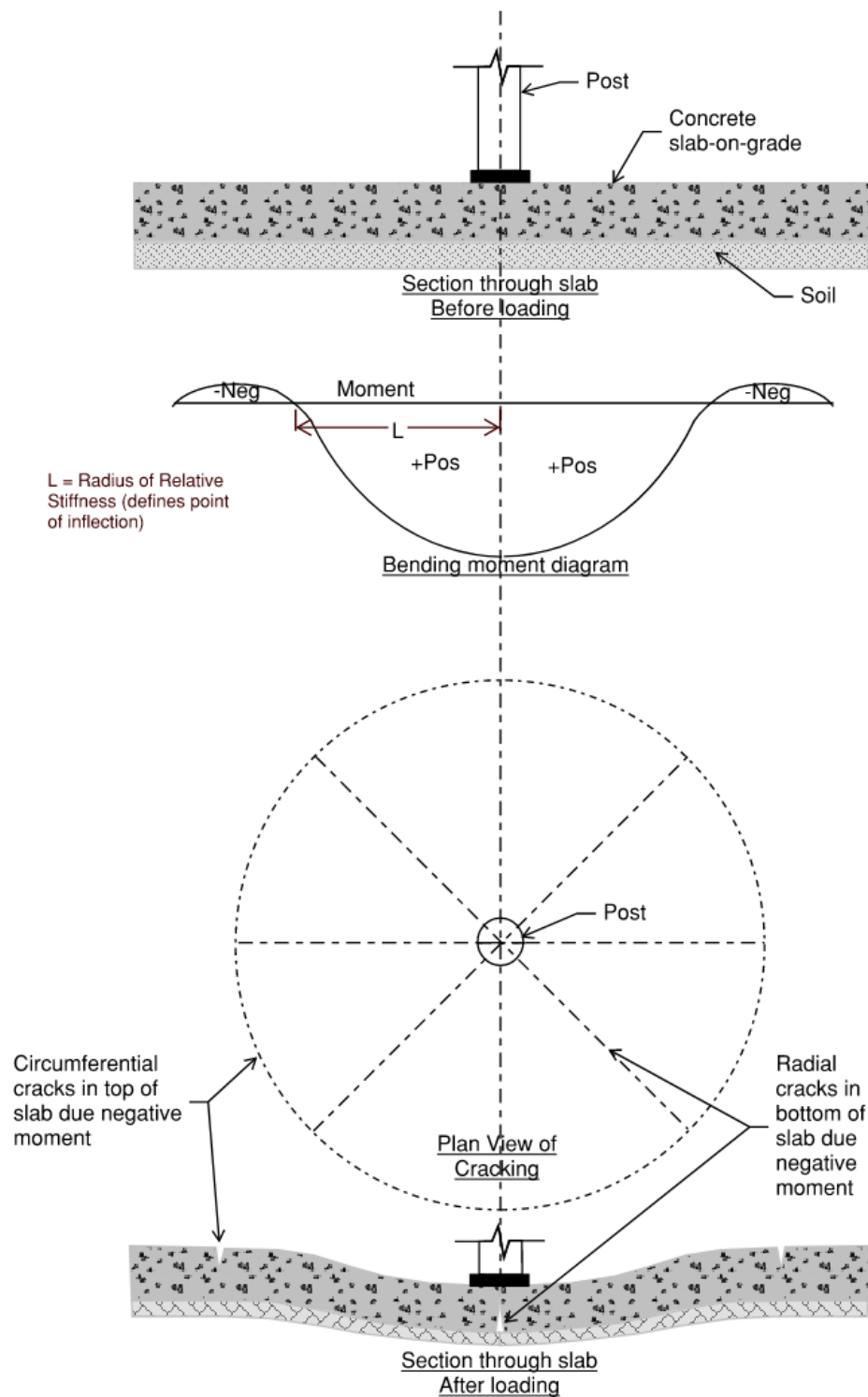
Fig. 31 – Slab cracking behavior due to a post load
