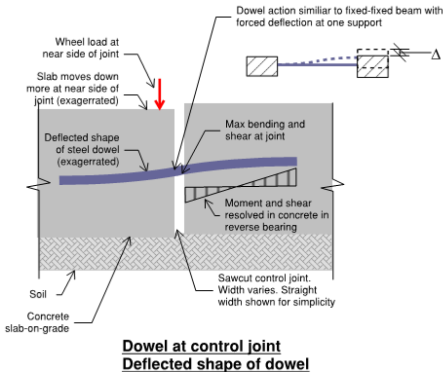
Fig. 40 - Diamond dowel action
