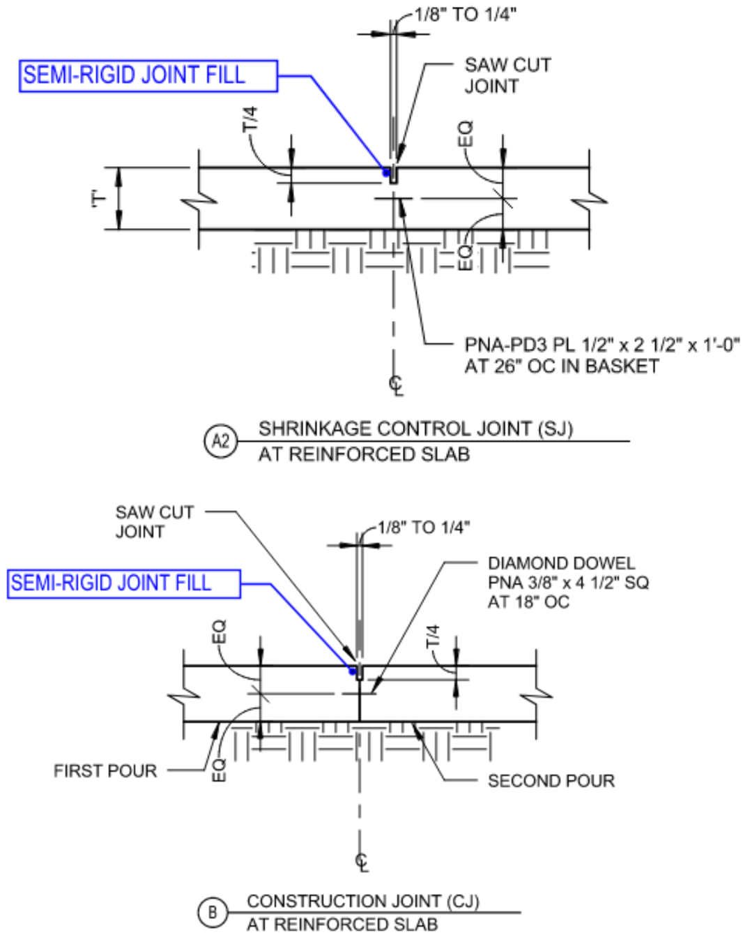
Fig. 48 - Slab-on-grade joint details
