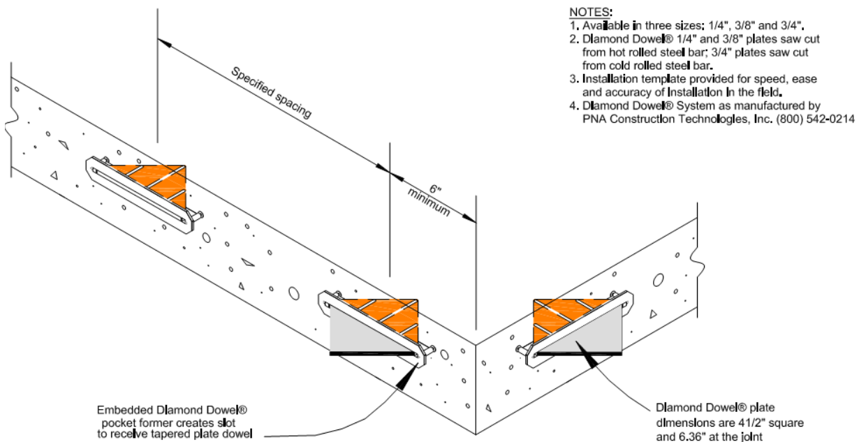
Fig 38 - Diamond dowels by PNA
