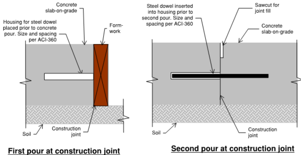
Fig. 39 – Diamond dowel placement
