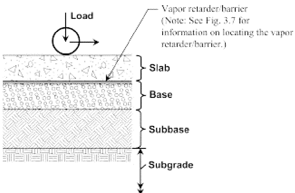
Fig. 29 – Slab-on-grade profile with soil– ACI 360
