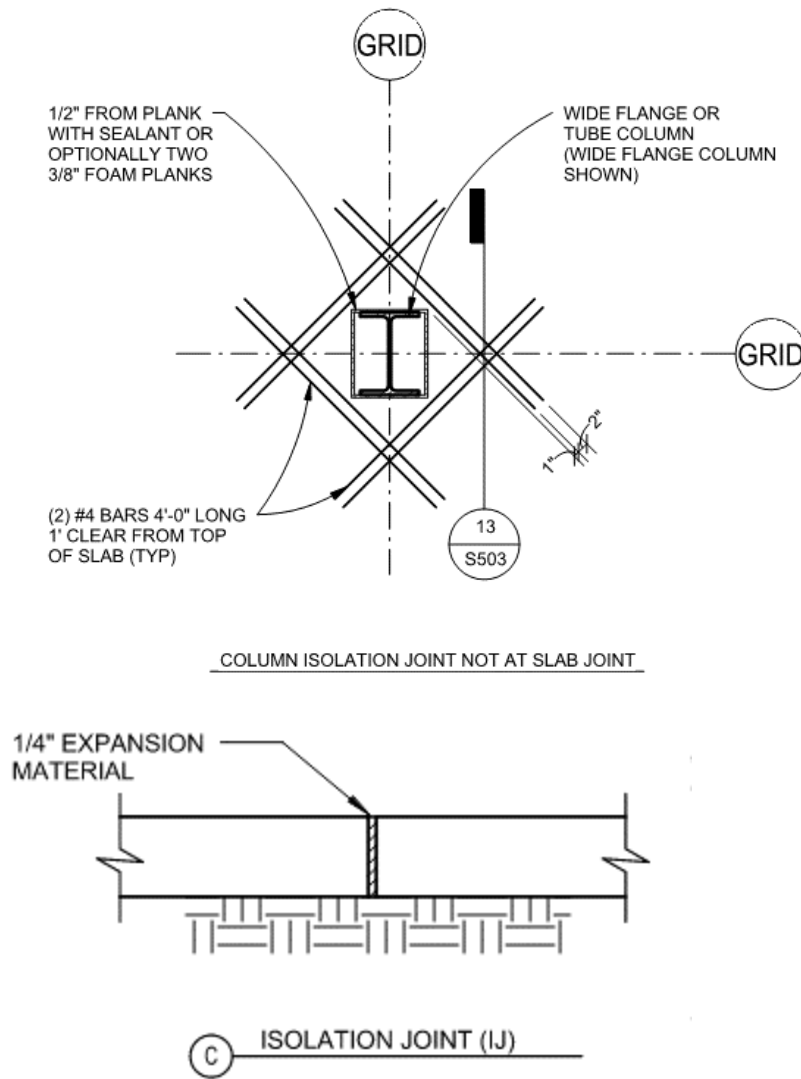
Fig. 49 - Details for typical isolation joints
