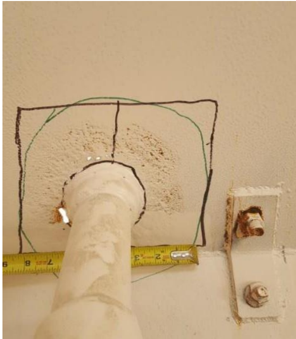
Figure 42: Thin steel discovered near a pipe penetration. The extent of the recommended reinforcing plate is drawn in black marker. In this case, two C-shaped plates are required.
