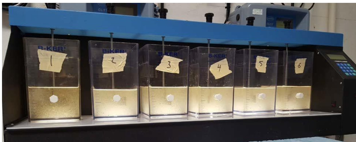
Figure 31: Jar testing with a gang stirrer and six influent samples, each with different chemical dosages. After 30 minutes, supernatant turbidity was measured for each.
