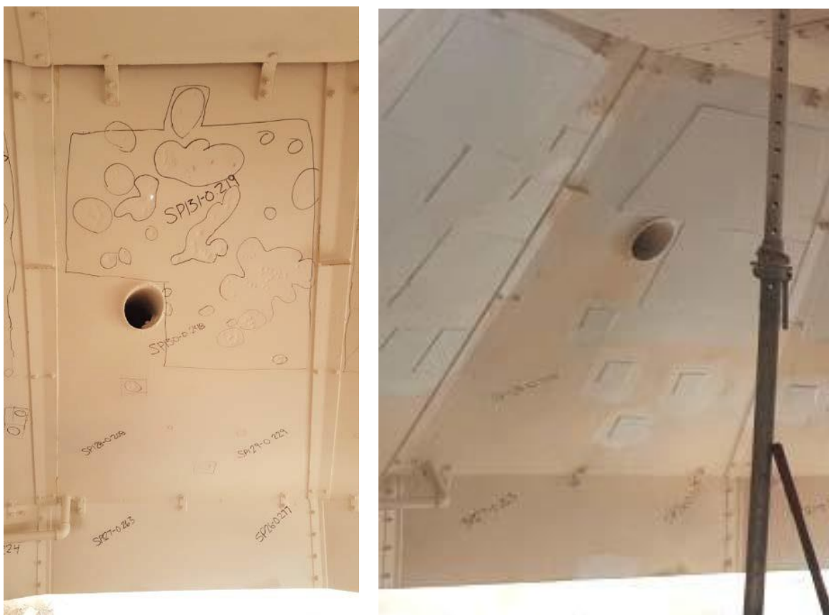
Figure 43: On left: Plate with thin areas delineated with black circles and the extents of the reinforcing areas drawn in black lines. Right: After reinforcing plates were welded to cover the thin areas.
