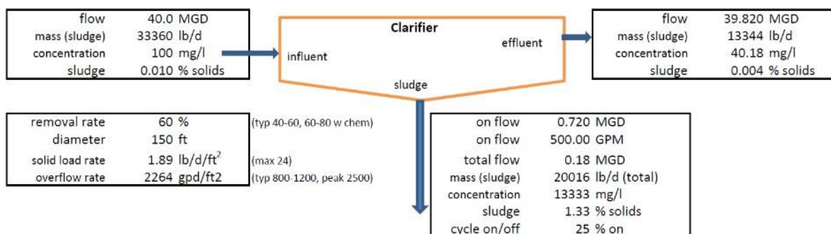
Figure 26: Example mass balance for a primary clarifier at peak flow. Note the mass of sludge entering the clarifier (33,360 lb/d) equals the mass leaving the clarifier (13,344 lb/d in effluent plus 20,016 lb/d in sludge).
