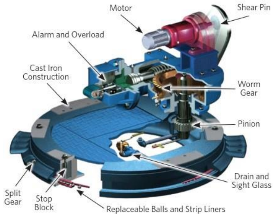
Figure 13: Center pier supported drive with major components identified
