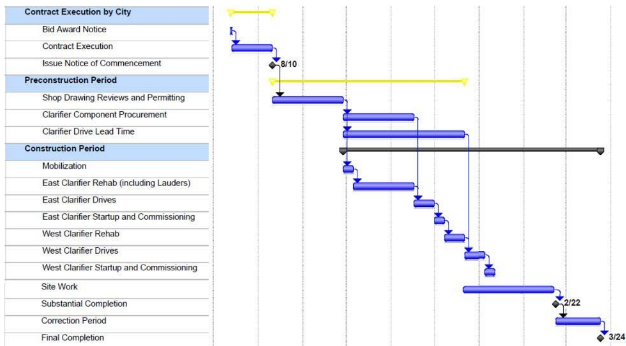
Figure 38: An overall construction schedule for a clarifier rehabilitation project. The clarifier rehab line items should be broken up into smaller tasks.
