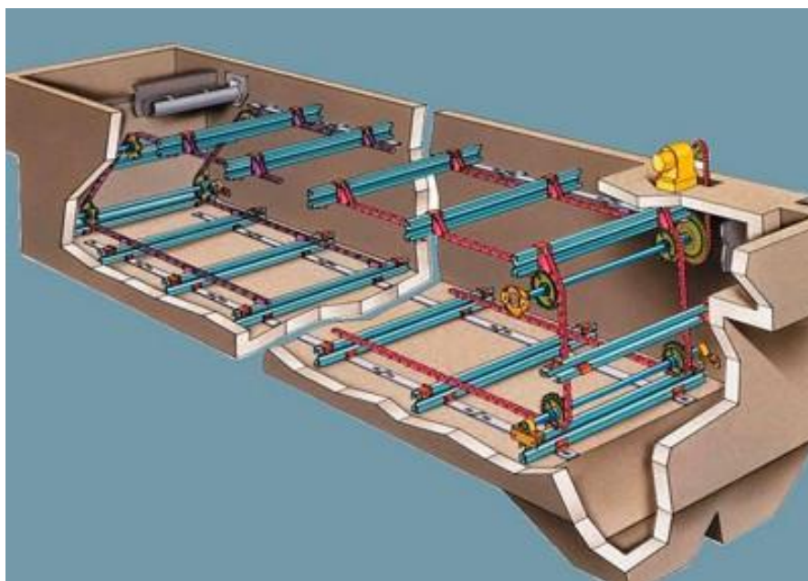
Figure 6: Rectangular clarifier components, including the chain (red), flights (blue), drive (yellow), sprockets (orange), and scum pipe (grey). The depressed chamber on the lower right is the sludge hopper.
