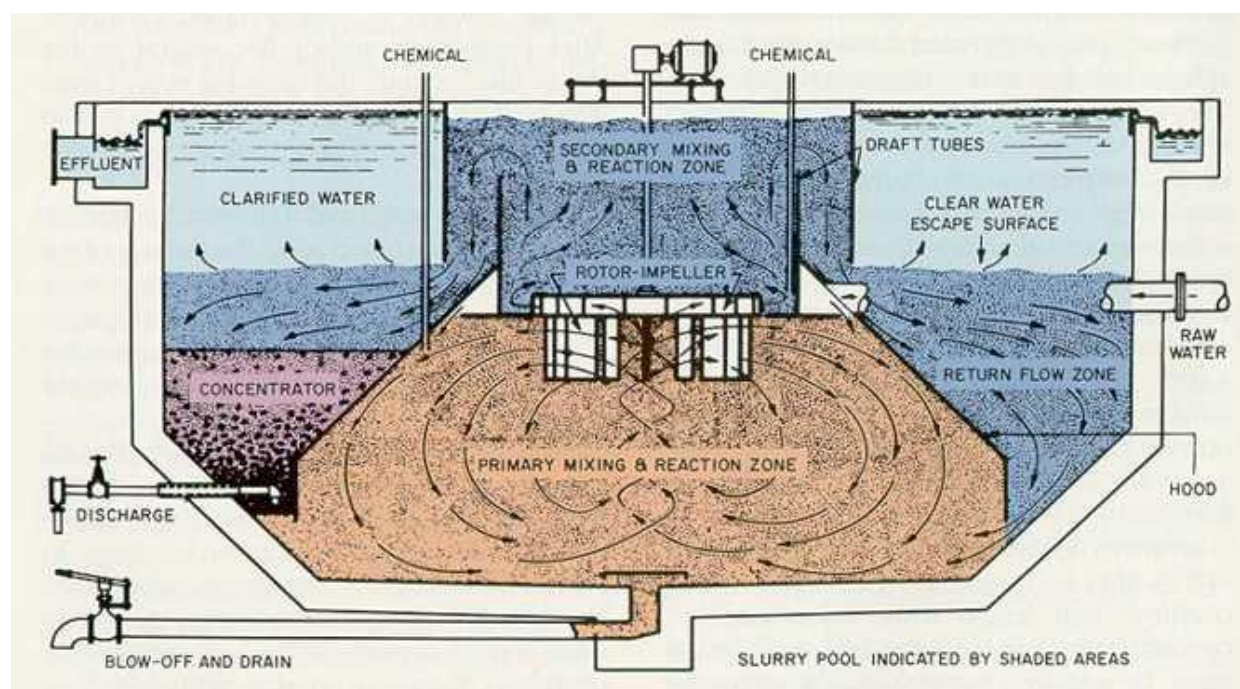
Figure 9: Zones in a typical solids contact clarifier.
