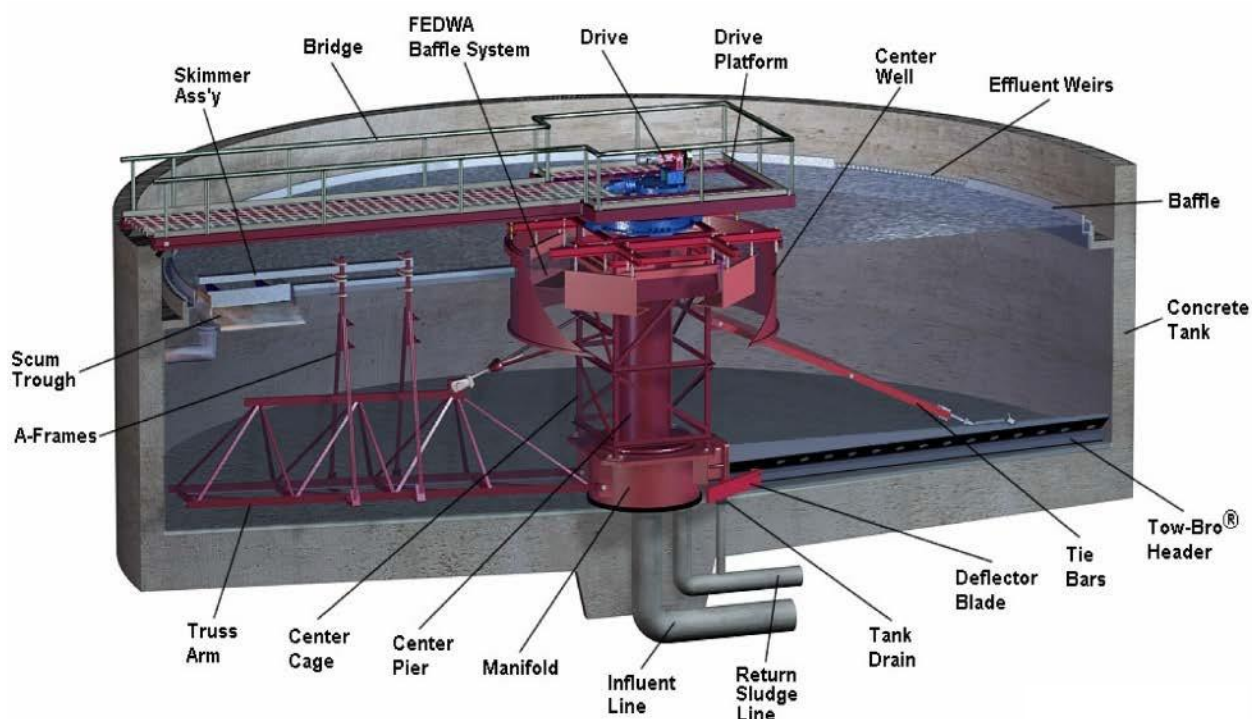
Figure 2: Typical components of a circular clarifier.
