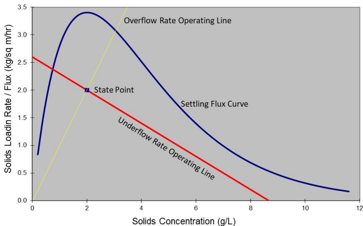
Figure 27: State point analysis chart with labels for the three plotted lines.
