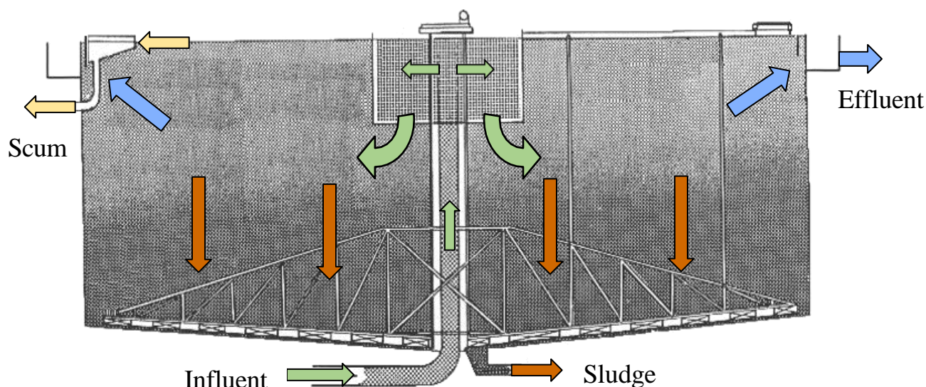
Figure 1: Flows in and out of a typical circular clarifier.
