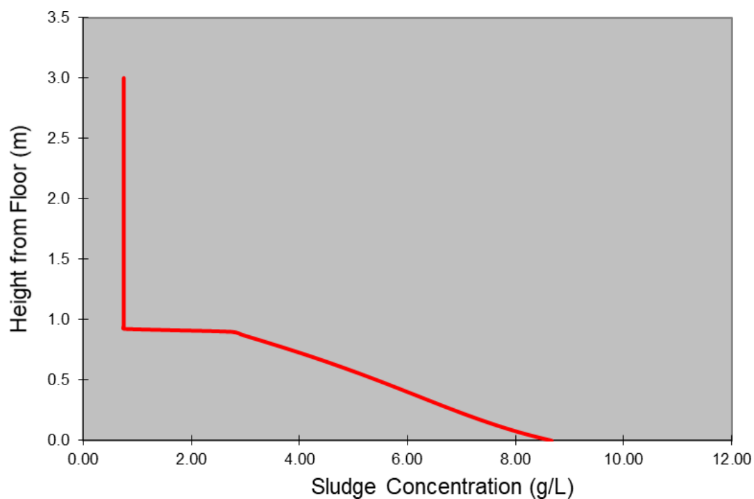
Figure 30: Example vertical solids profile for a gravity thickener.
