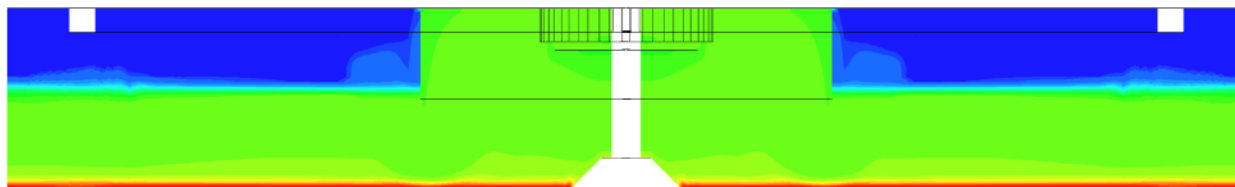
Figure 28: CFD model results for solids concentration of a secondary clarifier. Colors are as follows: dark blue is 10 mg/L, light blue is 1,000 mg/L, green is 3,000 mg/L, and red is 6,000 mg/L.
