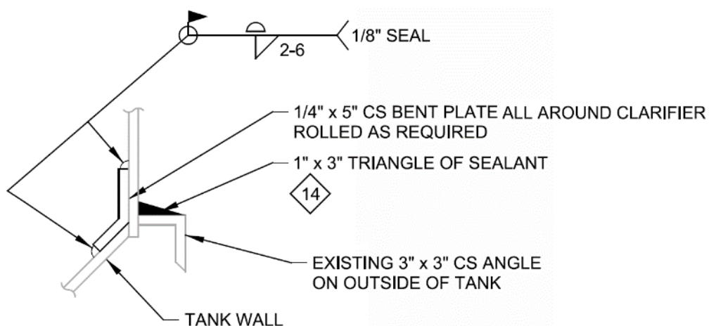
Figure 34: Example detail for adding a reinforcing plate and sealant to a tank wall.
